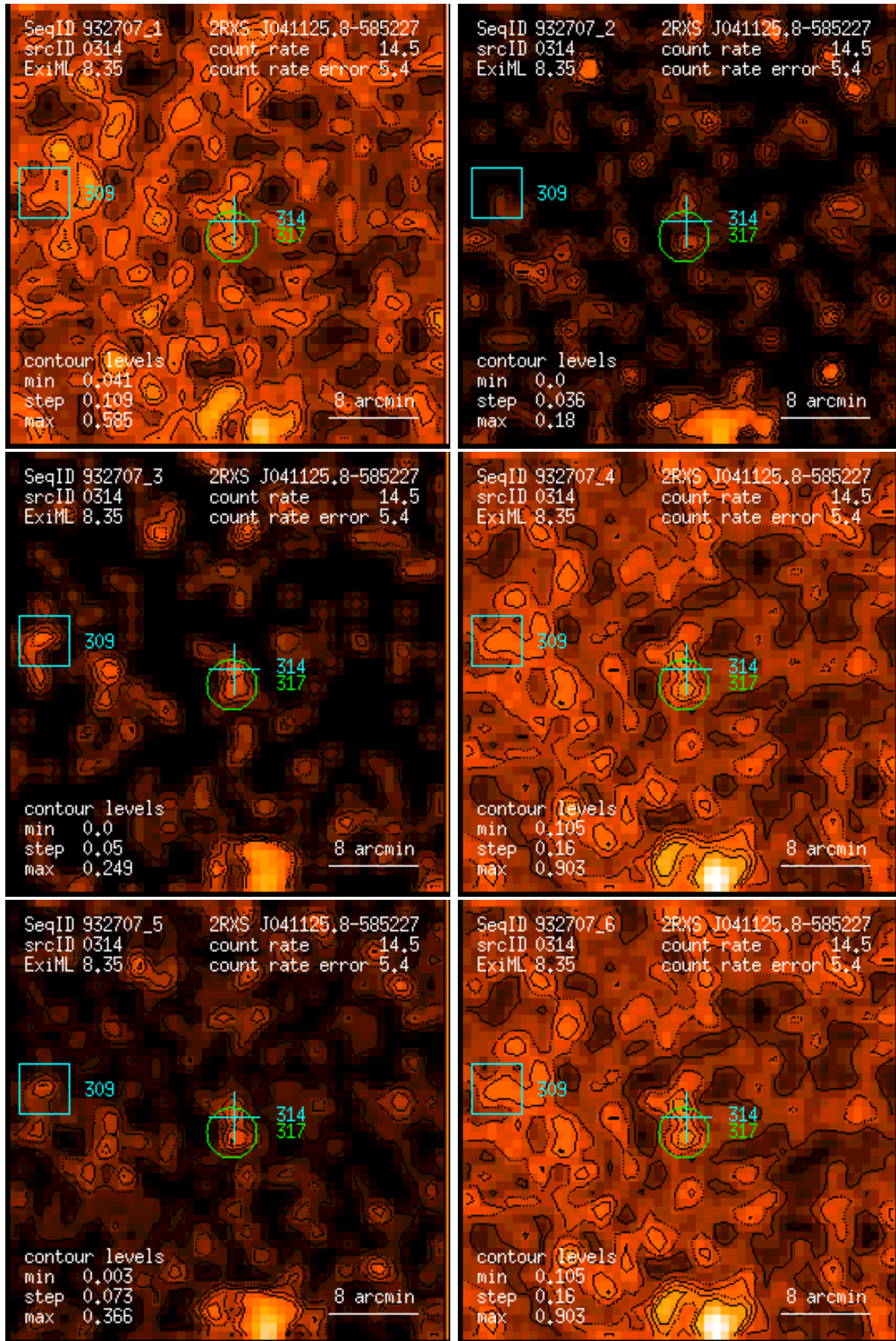
Figure 314: RASS 932707: detection 0314: band rate images, Gaussian filter: (1) PSPC channels 11 – 41, (2) 52 – 90, (3) 91 – 201, (4) 11 – 235, (5) 52 – 201, (6) 11 – 201. Broad band rates in counts/ks. Band rate contour levels in counts/ks/arcmin 2 .
