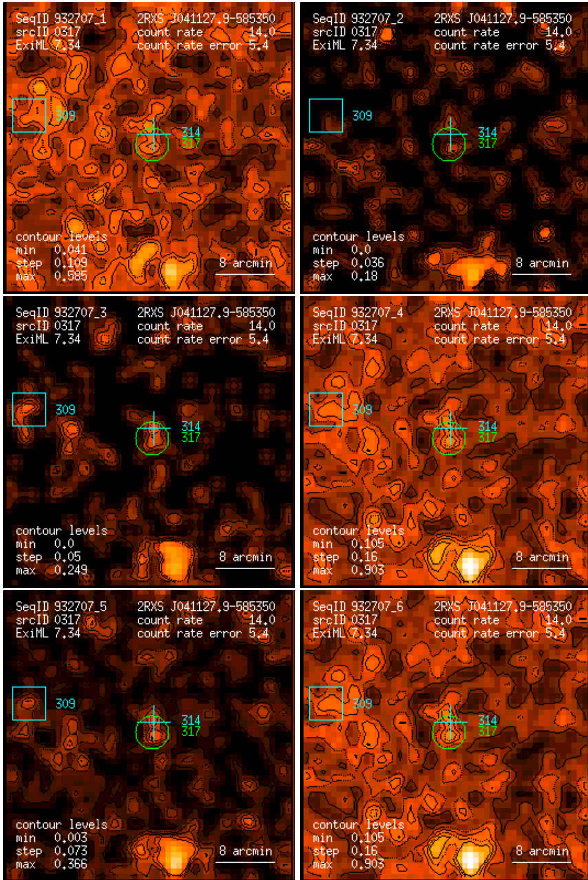
Figure 317: RASS 932707: detection 0317: band rate images, Gaussian filter: (1) PSPC channels 11 – 41, (2) 52 – 90, (3) 91 – 201, (4) 11 – 235, (5) 52 – 201, (6) 11 – 201. Broad band rates in counts/ks. Band rate contour levels in counts/ks/arcmin 2 .
