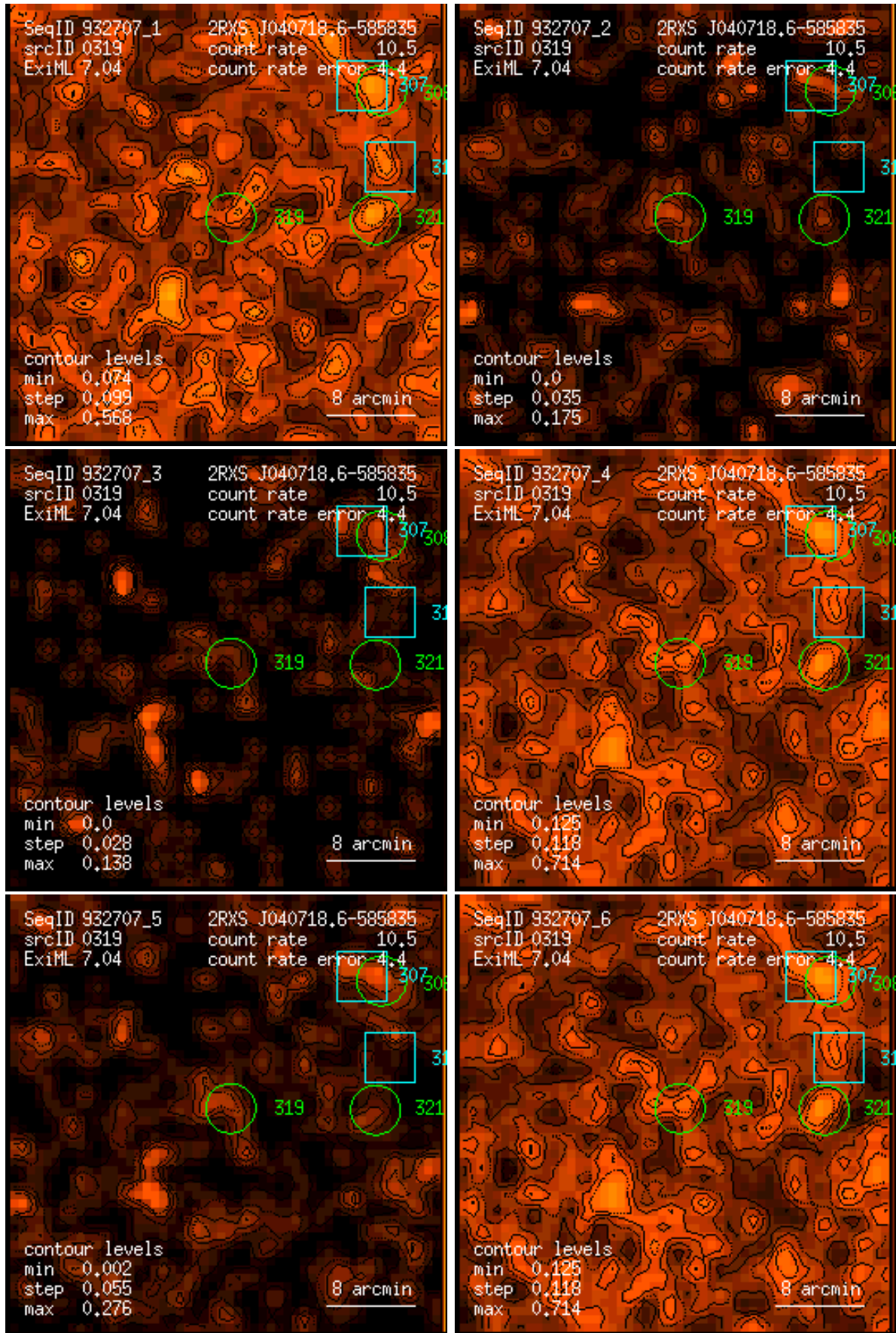
Figure 319: RASS 932707: detection 0319: band rate images, Gaussian filter: (1) PSPC channels 11 – 41, (2) 52 – 90, (3) 91 – 201, (4) 11 – 235, (5) 52 – 201, (6) 11 – 201. Broad band rates in counts/ks. Band rate contour levels in counts/ks/arcmin 2 .
