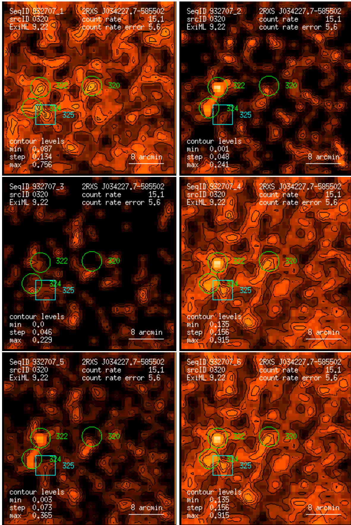
Figure 320: RASS 932707: detection 0320: band rate images, Gaussian filter: (1) PSPC channels 11 – 41, (2) 52 – 90, (3) 91 – 201, (4) 11 – 235, (5) 52 – 201, (6) 11 – 201. Broad band rates in counts/ks. Band rate contour levels in counts/ks/arcmin 2 .
