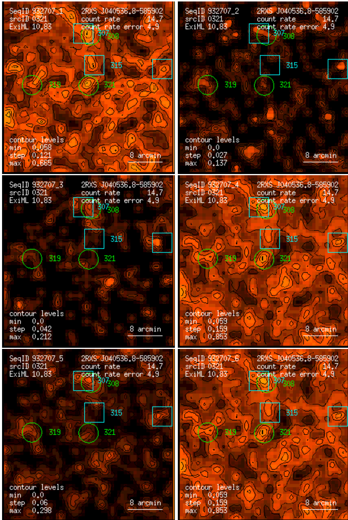
Figure 321: RASS 932707: detection 0321: band rate images, Gaussian filter: (1) PSPC channels 11 – 41, (2) 52 – 90, (3) 91 – 201, (4) 11 – 235, (5) 52 – 201, (6) 11 – 201. Broad band rates in counts/ks. Band rate contour levels in counts/ks/arcmin 2 .
