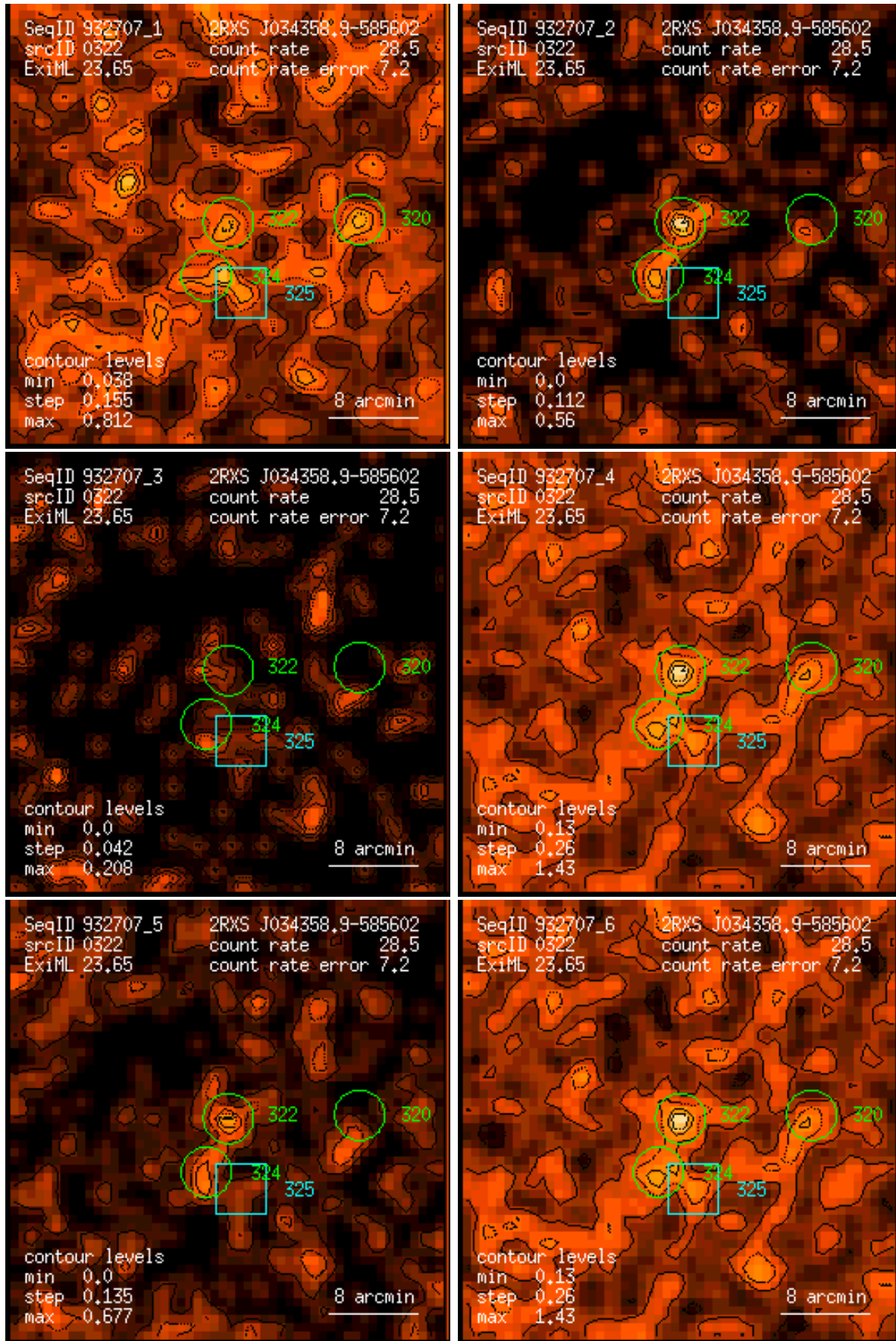
Figure 322: RASS 932707: detection 0322: band rate images, Gaussian filter: (1) PSPC channels 11 – 41, (2) 52 – 90, (3) 91 – 201, (4) 11 – 235, (5) 52 – 201, (6) 11 – 201. Broad band rates in counts/ks. Band rate contour levels in counts/ks/arcmin 2 .
