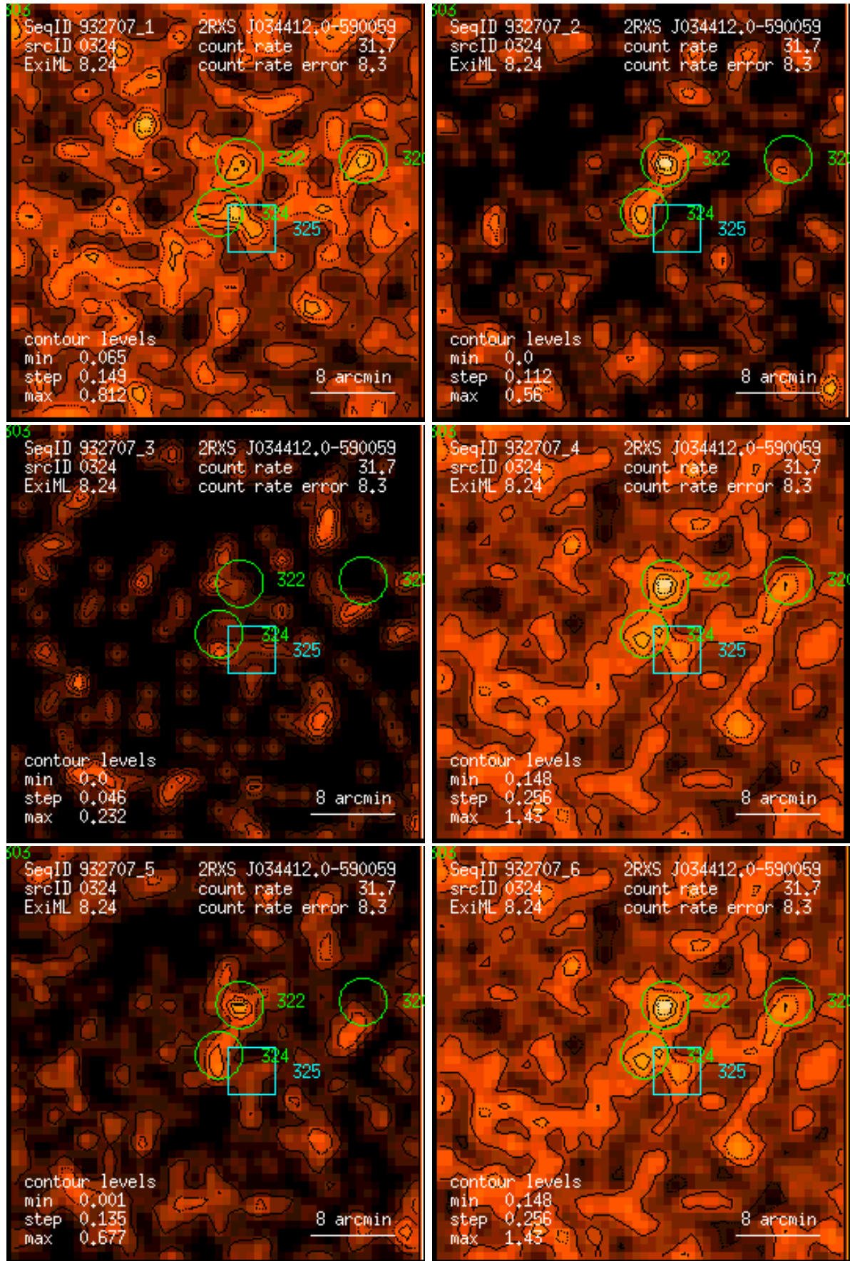
Figure 324: RASS 932707: detection 0324: band rate images, Gaussian filter: (1) PSPC channels 11 – 41, (2) 52 – 90, (3) 91 – 201, (4) 11 – 235, (5) 52 – 201, (6) 11 – 201. Broad band rates in counts/ks. Band rate contour levels in counts/ks/arcmin 2 .
