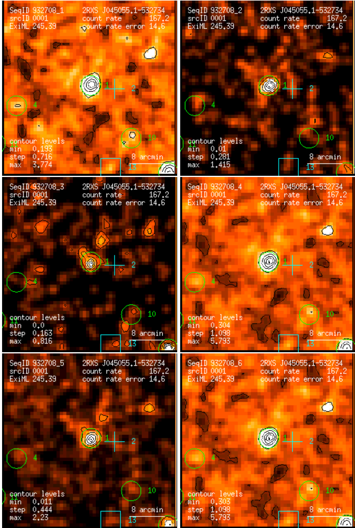
Figure 1: RASS 932708: detection 0001: band rate images, Gaussian filter: (1) PSPC channels 11 – 41, (2) 52 – 90, (3) 91 – 201, (4) 11 – 235, (5) 52 – 201, (6) 11 – 201. Broad band rates in counts/ks. Band rate contour levels in counts/ks/arcmin 2 .
