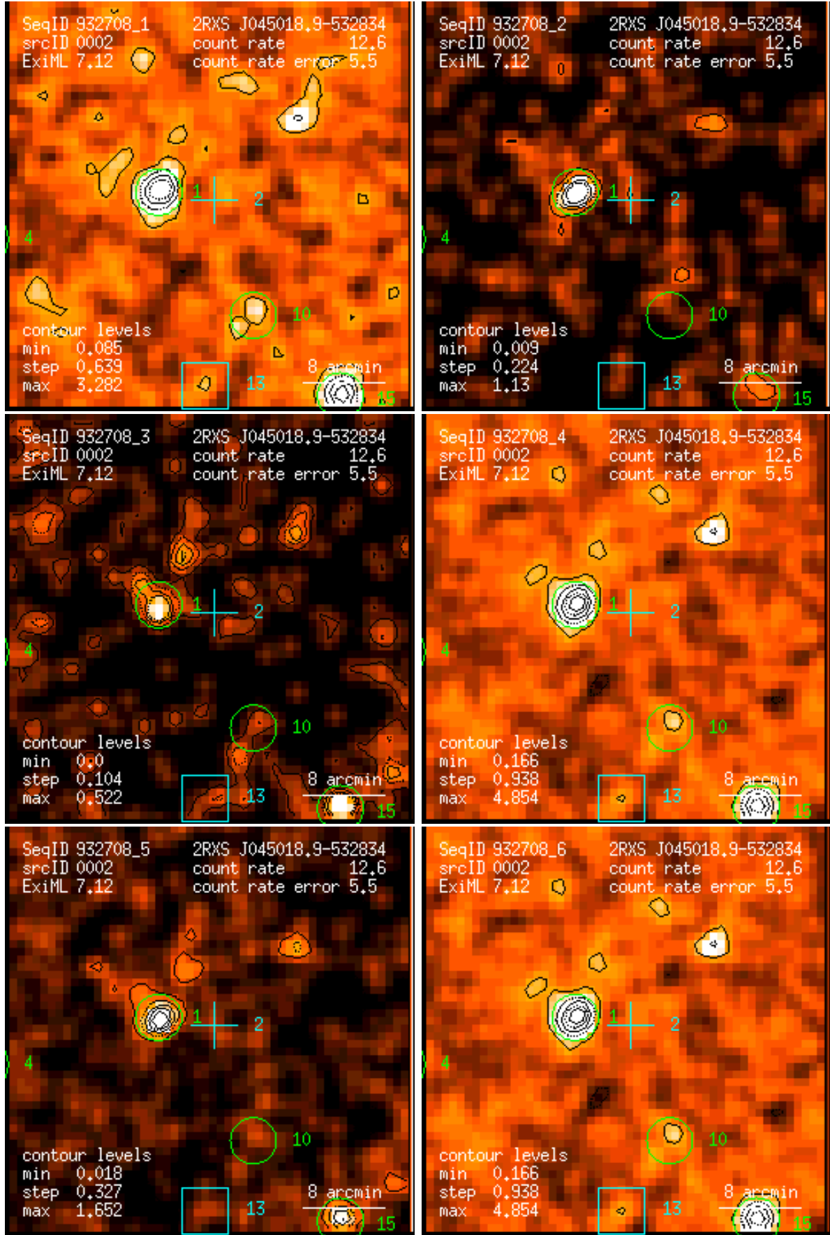
Figure 2: RASS 932708: detection 0002: band rate images, Gaussian filter: (1) PSPC channels 11 – 41, (2) 52 – 90, (3) 91 – 201, (4) 11 – 235, (5) 52 – 201, (6) 11 – 201. Broad band rates in counts/ks. Band rate contour levels in counts/ks/arcmin 2 .
