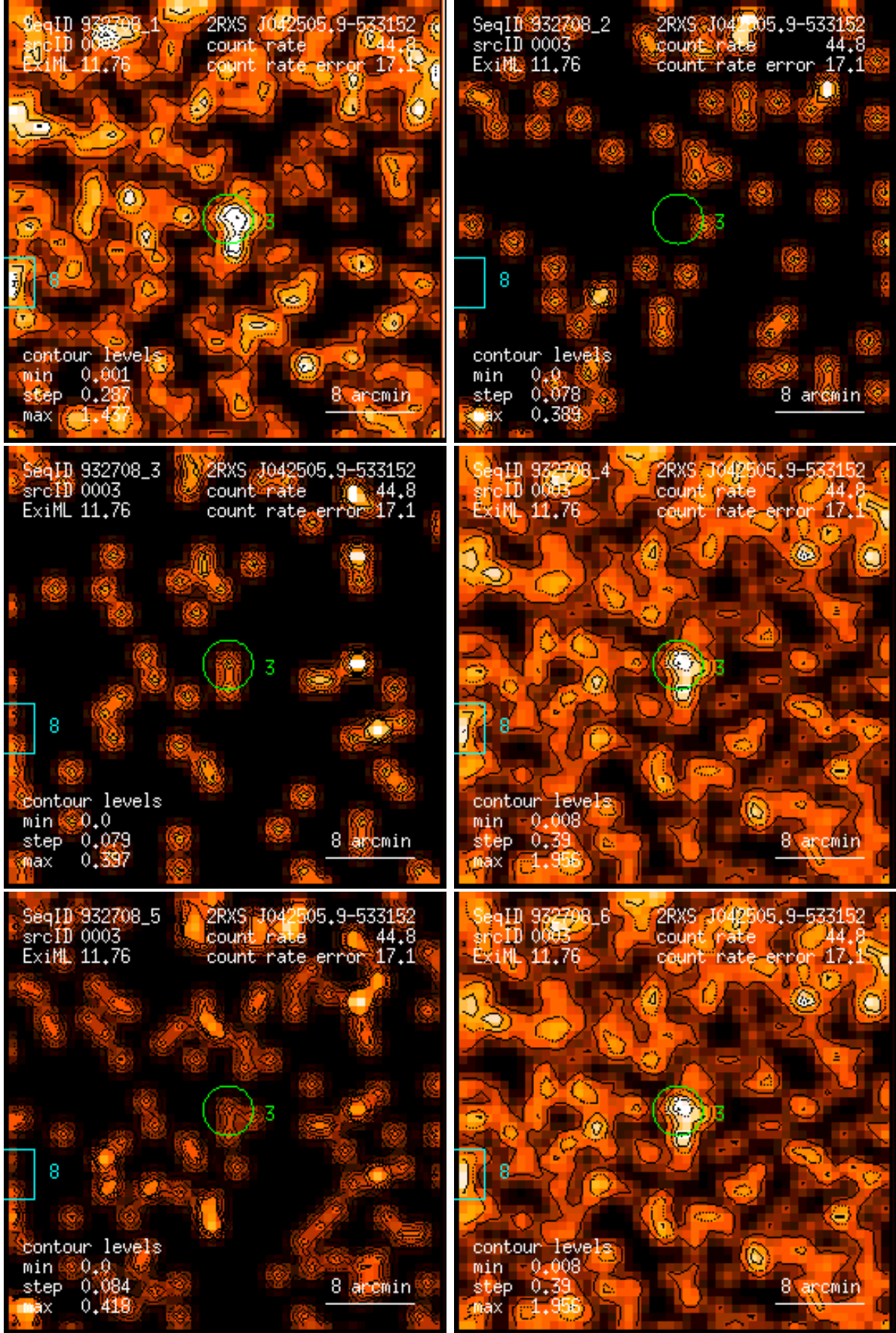
Figure 3: RASS 932708: detection 0003: band rate images, Gaussian filter: (1) PSPC channels 11 – 41, (2) 52 – 90, (3) 91 – 201, (4) 11 – 235, (5) 52 – 201, (6) 11 – 201. Broad band rates in counts/ks. Band rate contour levels in counts/ks/arcmin 2 .
