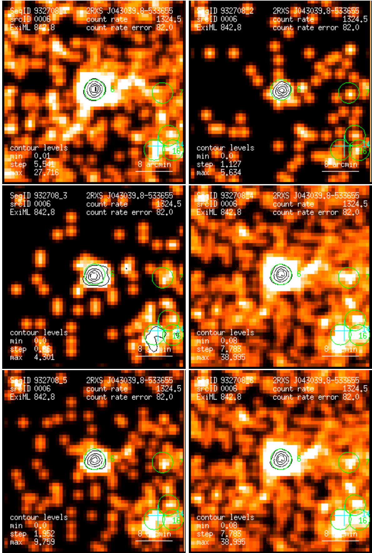
Figure 6: RASS 932708: detection 0006: band rate images, Gaussian filter: (1) PSPC channels 11 – 41, (2) 52 – 90, (3) 91 – 201, (4) 11 – 235, (5) 52 – 201, (6) 11 – 201. Broad band rates in counts/ks. Band rate contour levels in counts/ks/arcmin 2 .
