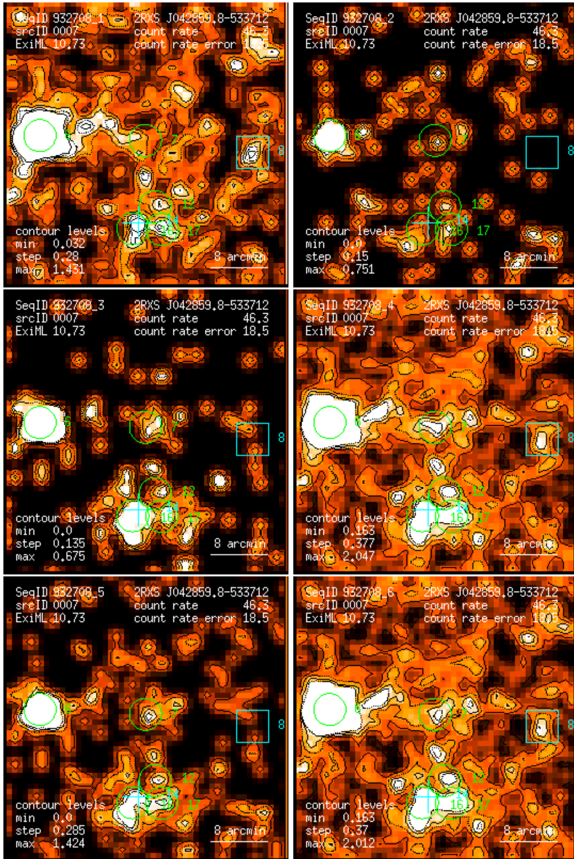
Figure 7: RASS 932708: detection 0007: band rate images, Gaussian filter: (1) PSPC channels 11 – 41, (2) 52 – 90, (3) 91 – 201, (4) 11 – 235, (5) 52 – 201, (6) 11 – 201. Broad band rates in counts/ks. Band rate contour levels in counts/ks/arcmin 2 .
