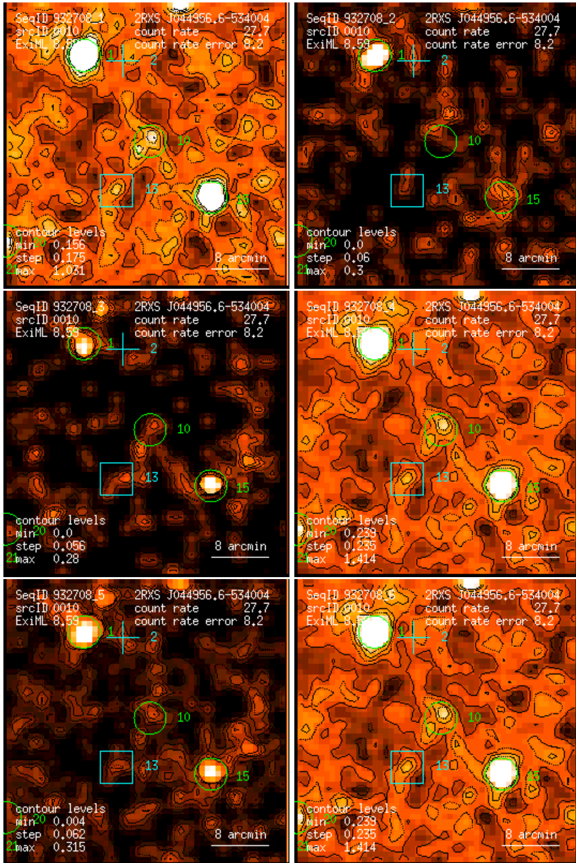
Figure 10: RASS 932708: detection 0010: band rate images, Gaussian filter: (1) PSPC channels 11 – 41, (2) 52 – 90, (3) 91 – 201, (4) 11 – 235, (5) 52 – 201, (6) 11 – 201. Broad band rates in counts/ks. Band rate contour levels in counts/ks/arcmin 2 .
