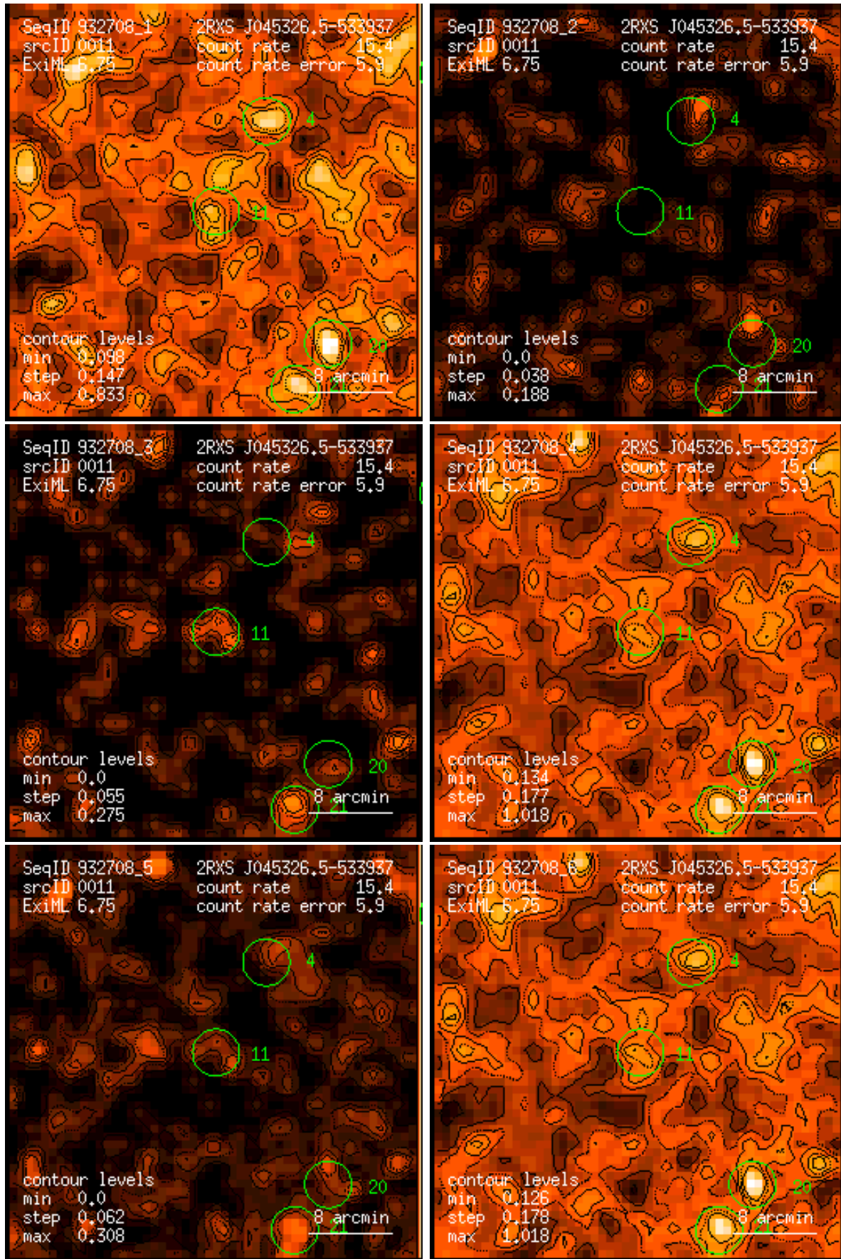
Figure 11: RASS 932708: detection 0011: band rate images, Gaussian filter: (1) PSPC channels 11 – 41, (2) 52 – 90, (3) 91 – 201, (4) 11 – 235, (5) 52 – 201, (6) 11 – 201. Broad band rates in counts/ks. Band rate contour levels in counts/ks/arcmin 2 .
