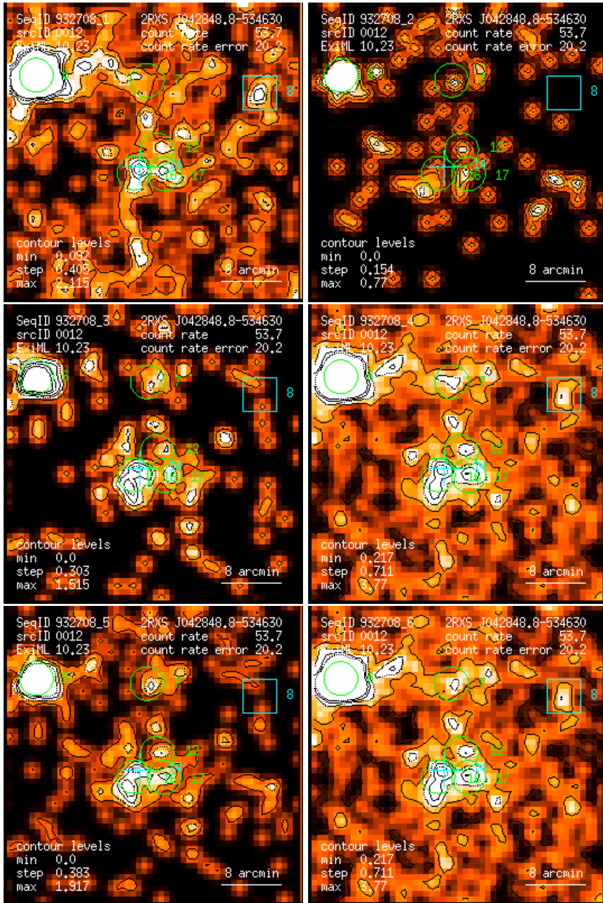
Figure 12: RASS 932708: detection 0012: band rate images, Gaussian filter: (1) PSPC channels 11 – 41, (2) 52 – 90, (3) 91 – 201, (4) 11 – 235, (5) 52 – 201, (6) 11 – 201. Broad band rates in counts/ks. Band rate contour levels in counts/ks/arcmin 2 .
