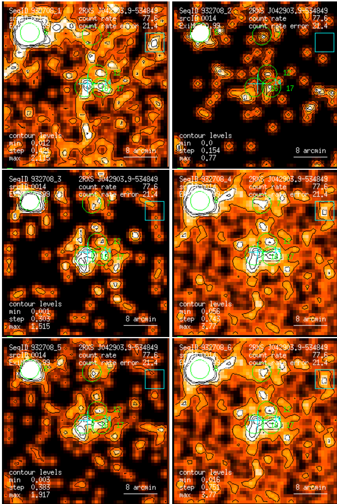
Figure 14: RASS 932708: detection 0014: band rate images, Gaussian filter: (1) PSPC channels 11 – 41, (2) 52 – 90, (3) 91 – 201, (4) 11 – 235, (5) 52 – 201, (6) 11 – 201. Broad band rates in counts/ks. Band rate contour levels in counts/ks/arcmin 2 .
