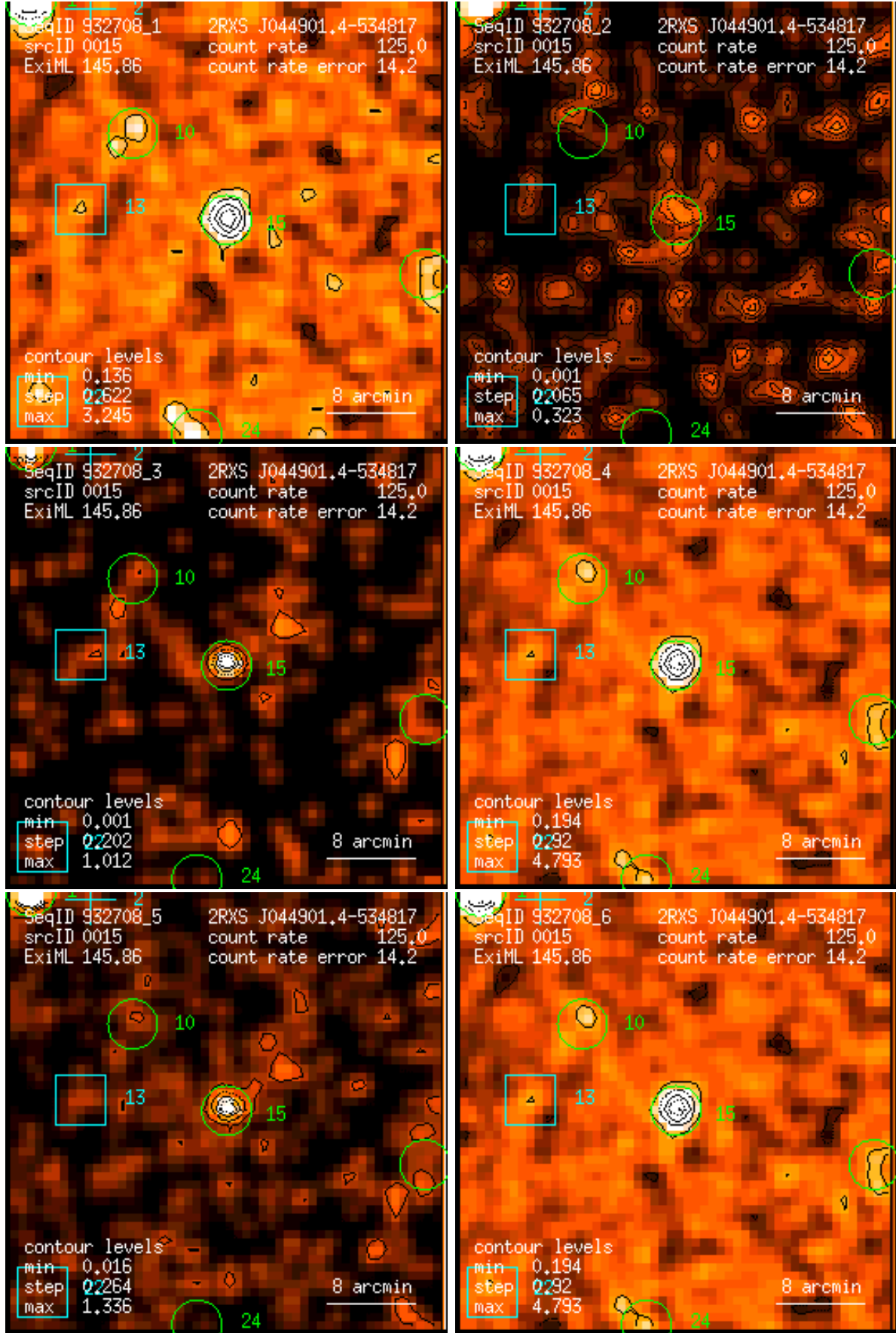
Figure 15: RASS 932708: detection 0015: band rate images, Gaussian filter: (1) PSPC channels 11 – 41, (2) 52 – 90, (3) 91 – 201, (4) 11 – 235, (5) 52 – 201, (6) 11 – 201. Broad band rates in counts/ks. Band rate contour levels in counts/ks/arcmin 2 .
