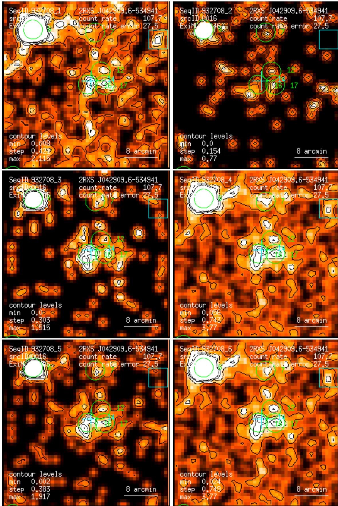
Figure 16: RASS 932708: detection 0016: band rate images, Gaussian filter: (1) PSPC channels 11 – 41, (2) 52 – 90, (3) 91 – 201, (4) 11 – 235, (5) 52 – 201, (6) 11 – 201. Broad band rates in counts/ks. Band rate contour levels in counts/ks/arcmin 2 .
