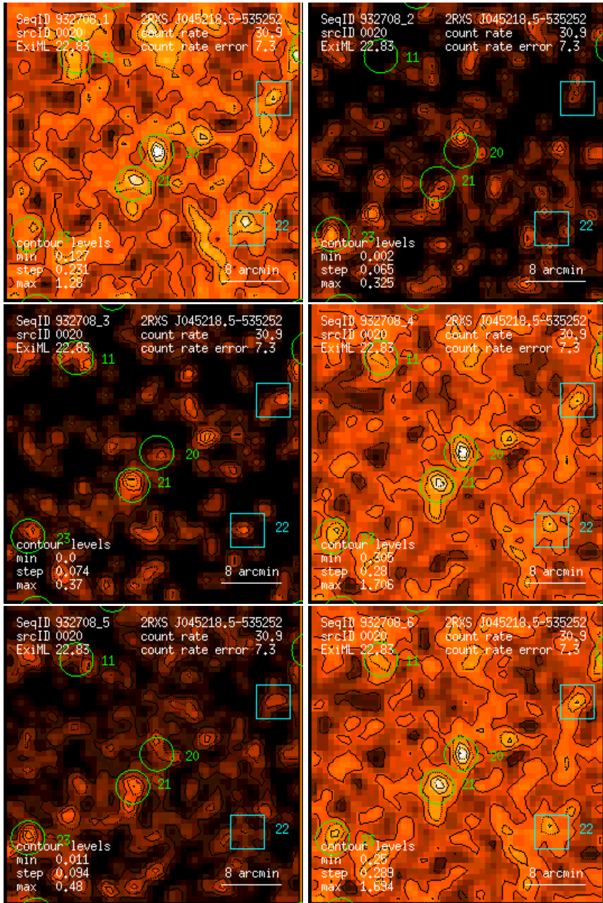
Figure 20: RASS 932708: detection 0020: band rate images, Gaussian filter: (1) PSPC channels 11 – 41, (2) 52 – 90, (3) 91 – 201, (4) 11 – 235, (5) 52 – 201, (6) 11 – 201. Broad band rates in counts/ks. Band rate contour levels in counts/ks/arcmin 2 .
