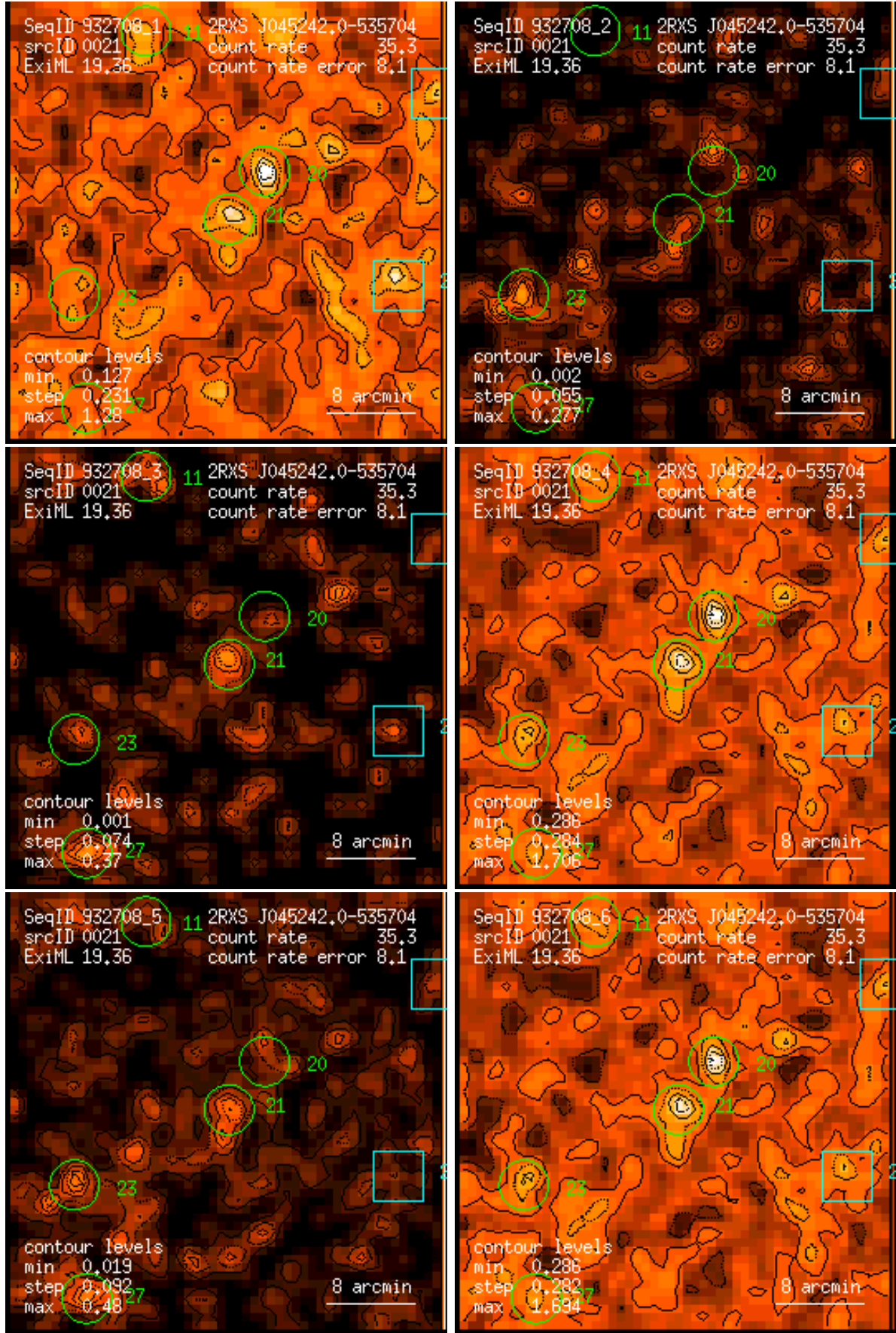
Figure 21: RASS 932708: detection 0021: band rate images, Gaussian filter: (1) PSPC channels 11 – 41, (2) 52 – 90, (3) 91 – 201, (4) 11 – 235, (5) 52 – 201, (6) 11 – 201. Broad band rates in counts/ks. Band rate contour levels in counts/ks/arcmin 2 .
