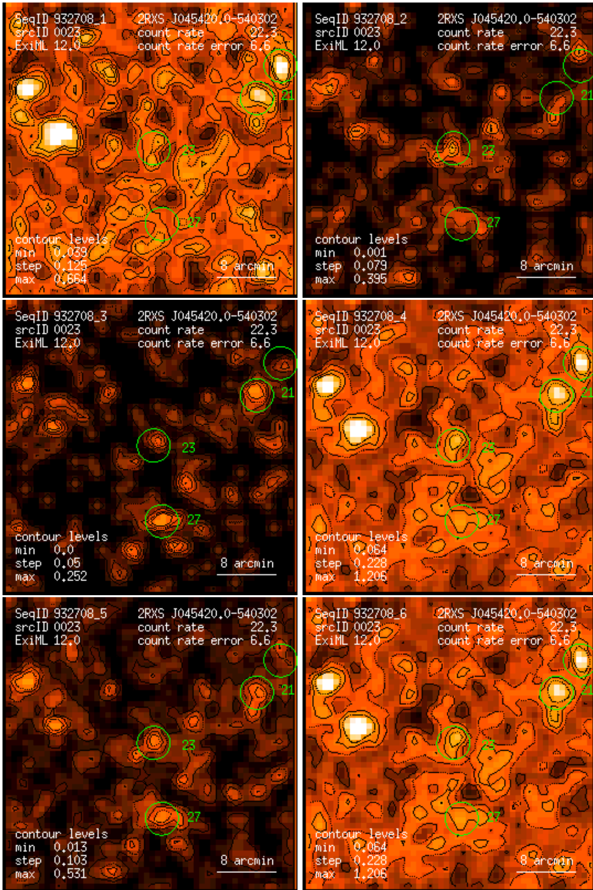
Figure 23: RASS 932708: detection 0023: band rate images, Gaussian filter: (1) PSPC channels 11 – 41, (2) 52 – 90, (3) 91 – 201, (4) 11 – 235, (5) 52 – 201, (6) 11 – 201. Broad band rates in counts/ks. Band rate contour levels in counts/ks/arcmin 2 .
