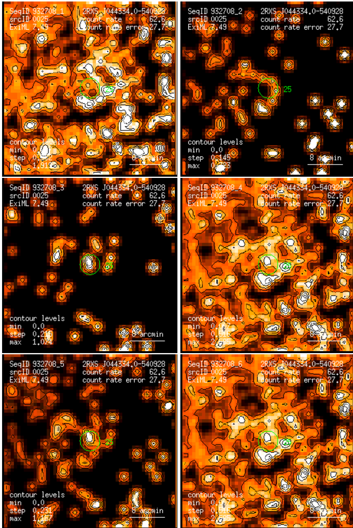
Figure 25: RASS 932708: detection 0025: band rate images, Gaussian filter: (1) PSPC channels 11 – 41, (2) 52 – 90, (3) 91 – 201, (4) 11 – 235, (5) 52 – 201, (6) 11 – 201. Broad band rates in counts/ks. Band rate contour levels in counts/ks/arcmin 2 .
