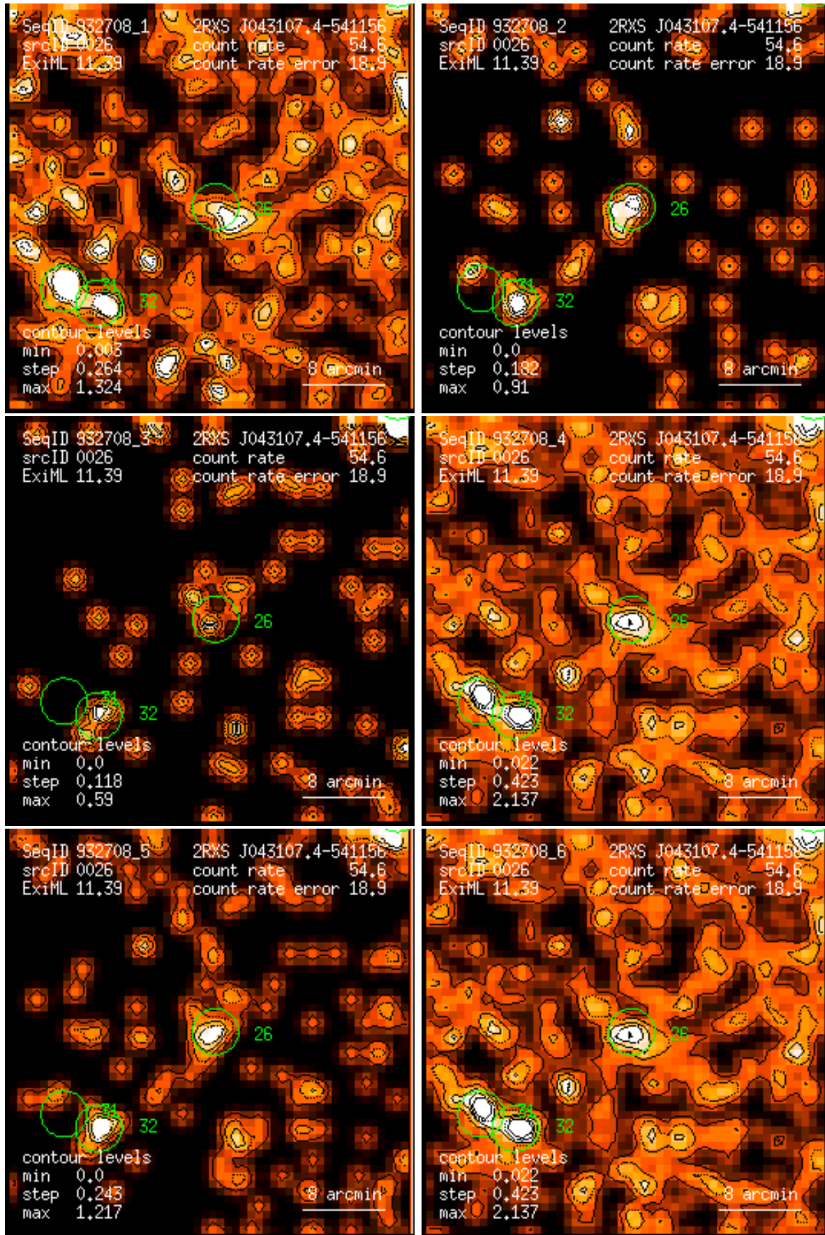
Figure 26: RASS 932708: detection 0026: band rate images, Gaussian filter: (1) PSPC channels 11 – 41, (2) 52 – 90, (3) 91 – 201, (4) 11 – 235, (5) 52 – 201, (6) 11 – 201. Broad band rates in counts/ks. Band rate contour levels in counts/ks/arcmin 2 .
