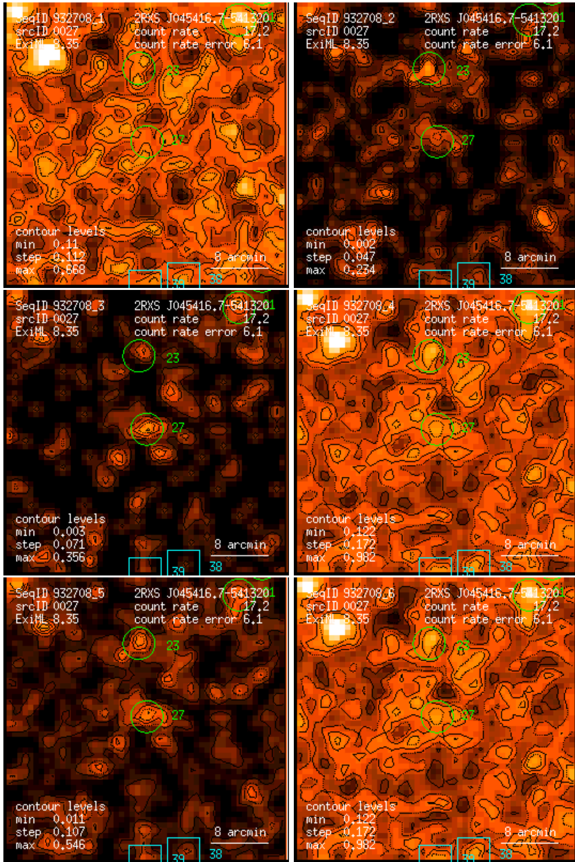
Figure 27: RASS 932708: detection 0027: band rate images, Gaussian filter: (1) PSPC channels 11 – 41, (2) 52 – 90, (3) 91 – 201, (4) 11 – 235, (5) 52 – 201, (6) 11 – 201. Broad band rates in counts/ks. Band rate contour levels in counts/ks/arcmin 2 .
