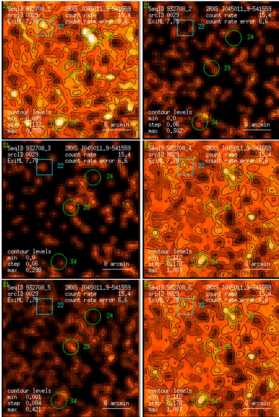
Figure 29: RASS 932708: detection 0029: band rate images, Gaussian filter: (1) PSPC channels 11 – 41, (2) 52 – 90, (3) 91 – 201, (4) 11 – 235, (5) 52 – 201, (6) 11 – 201. Broad band rates in counts/ks. Band rate contour levels in counts/ks/arcmin 2 .
