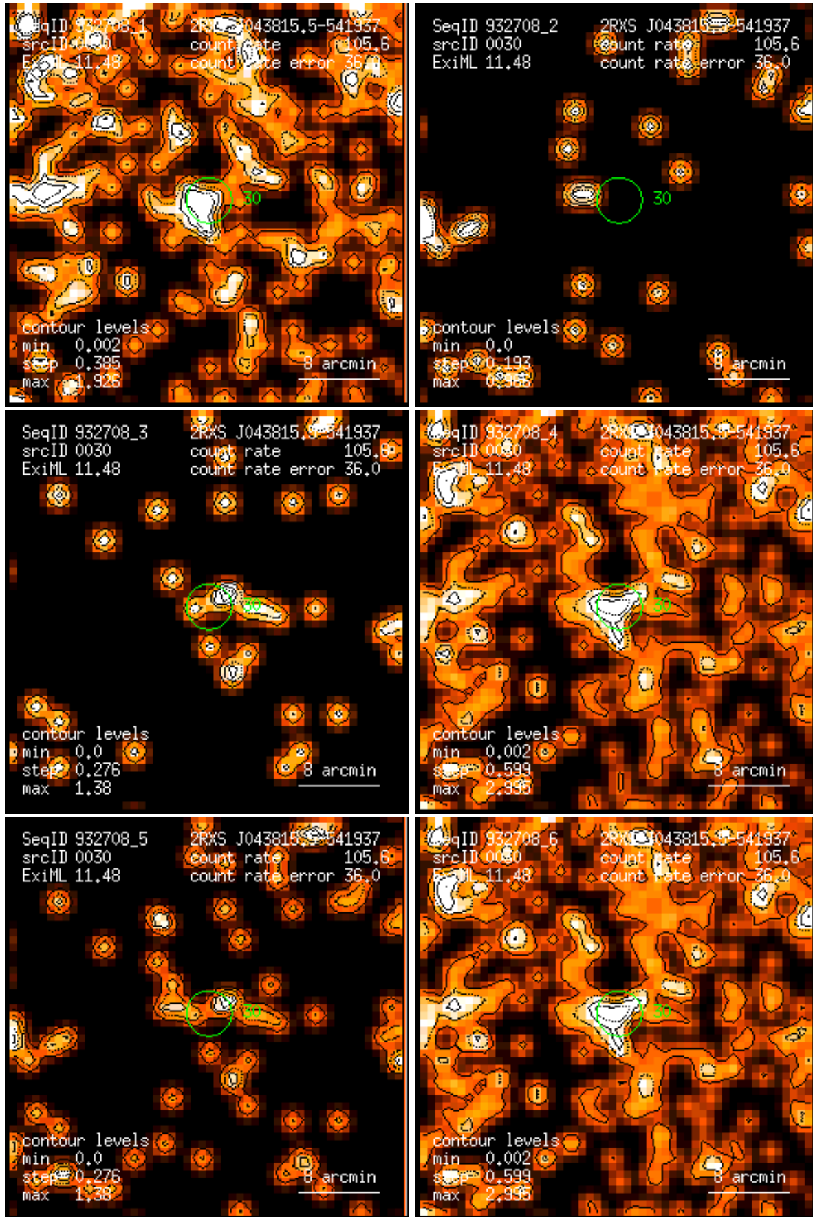
Figure 30: RASS 932708: detection 0030: band rate images, Gaussian filter: (1) PSPC channels 11 – 41, (2) 52 – 90, (3) 91 – 201, (4) 11 – 235, (5) 52 – 201, (6) 11 – 201. Broad band rates in counts/ks. Band rate contour levels in counts/ks/arcmin 2 .
