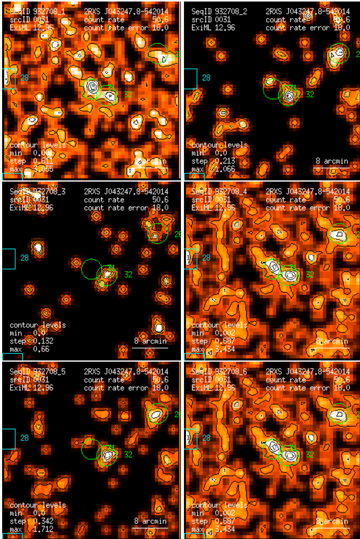
Figure 31: RASS 932708: detection 0031: band rate images, Gaussian filter: (1) PSPC channels 11 – 41, (2) 52 – 90, (3) 91 – 201, (4) 11 – 235, (5) 52 – 201, (6) 11 – 201. Broad band rates in counts/ks. Band rate contour levels in counts/ks/arcmin 2 .
