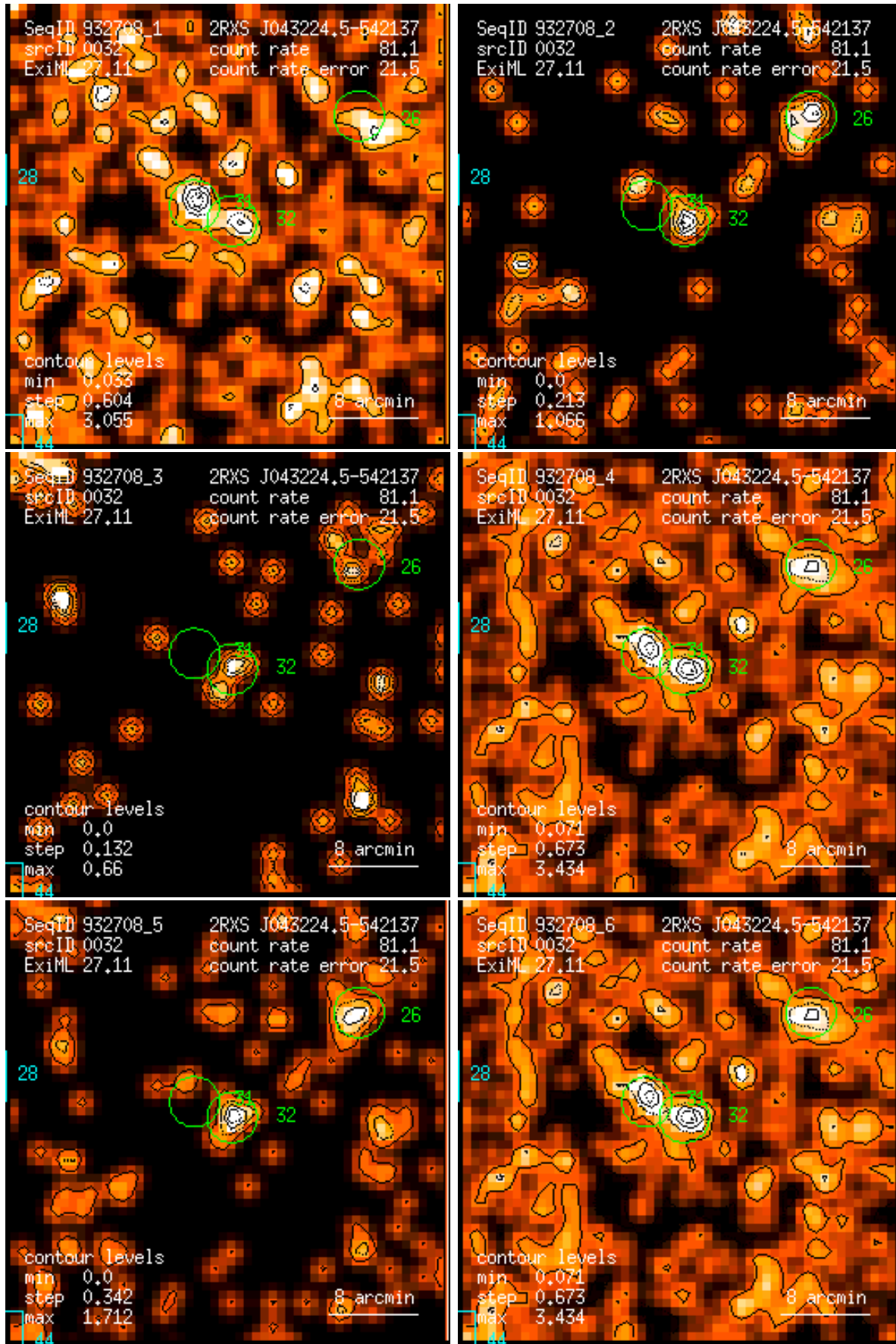
Figure 32: RASS 932708: detection 0032: band rate images, Gaussian filter: (1) PSPC channels 11 – 41, (2) 52 – 90, (3) 91 – 201, (4) 11 – 235, (5) 52 – 201, (6) 11 – 201. Broad band rates in counts/ks. Band rate contour levels in counts/ks/arcmin 2 .
