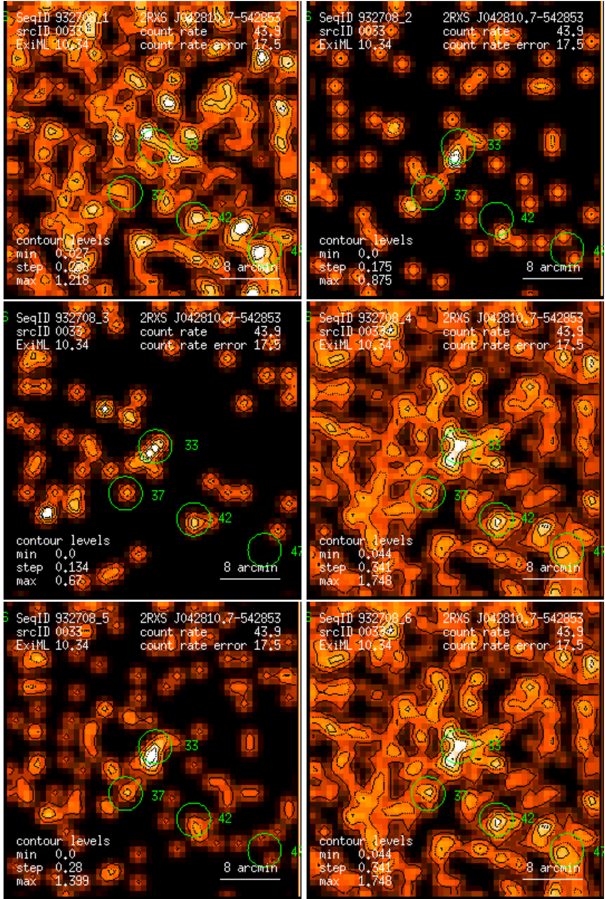
Figure 33: RASS 932708: detection 0033: band rate images, Gaussian filter: (1) PSPC channels 11 – 41, (2) 52 – 90, (3) 91 – 201, (4) 11 – 235, (5) 52 – 201, (6) 11 – 201. Broad band rates in counts/ks. Band rate contour levels in counts/ks/arcmin 2 .
