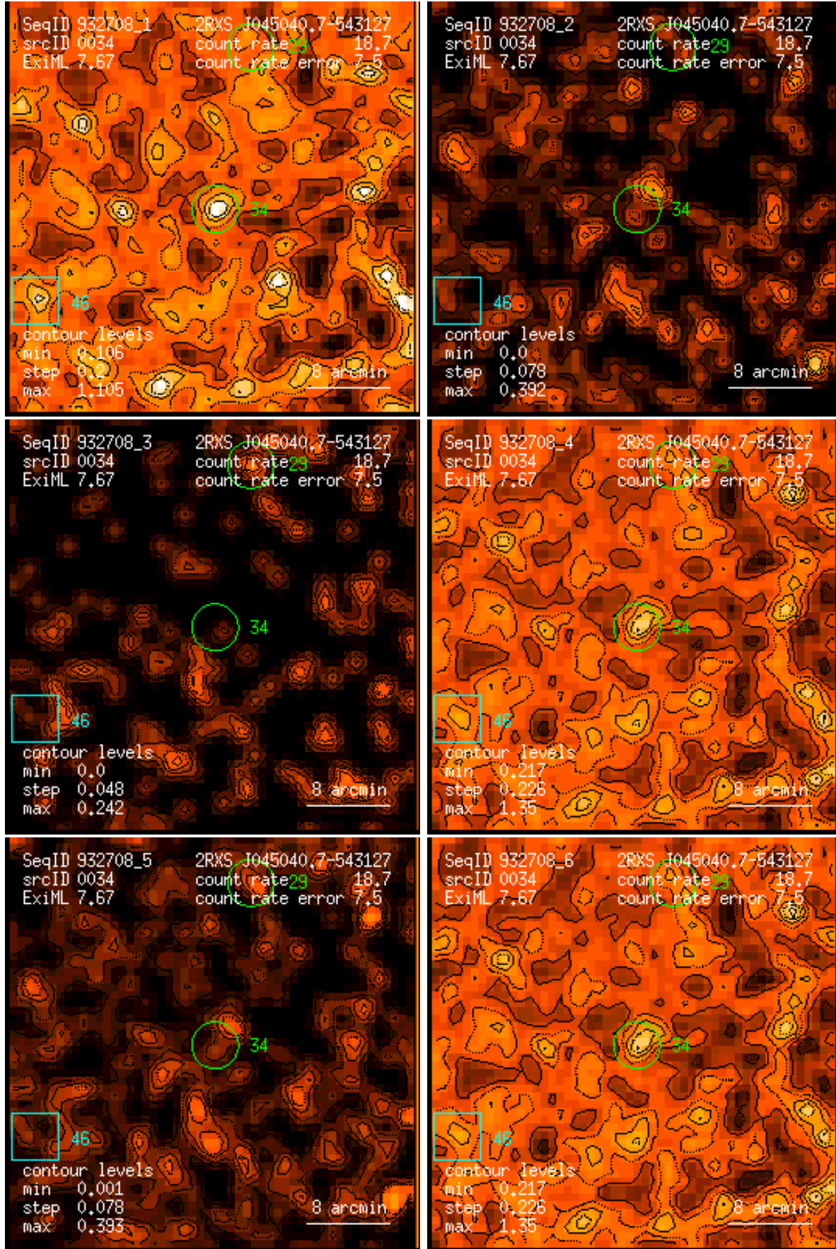
Figure 34: RASS 932708: detection 0034: band rate images, Gaussian filter: (1) PSPC channels 11 – 41, (2) 52 – 90, (3) 91 – 201, (4) 11 – 235, (5) 52 – 201, (6) 11 – 201. Broad band rates in counts/ks. Band rate contour levels in counts/ks/arcmin 2 .
