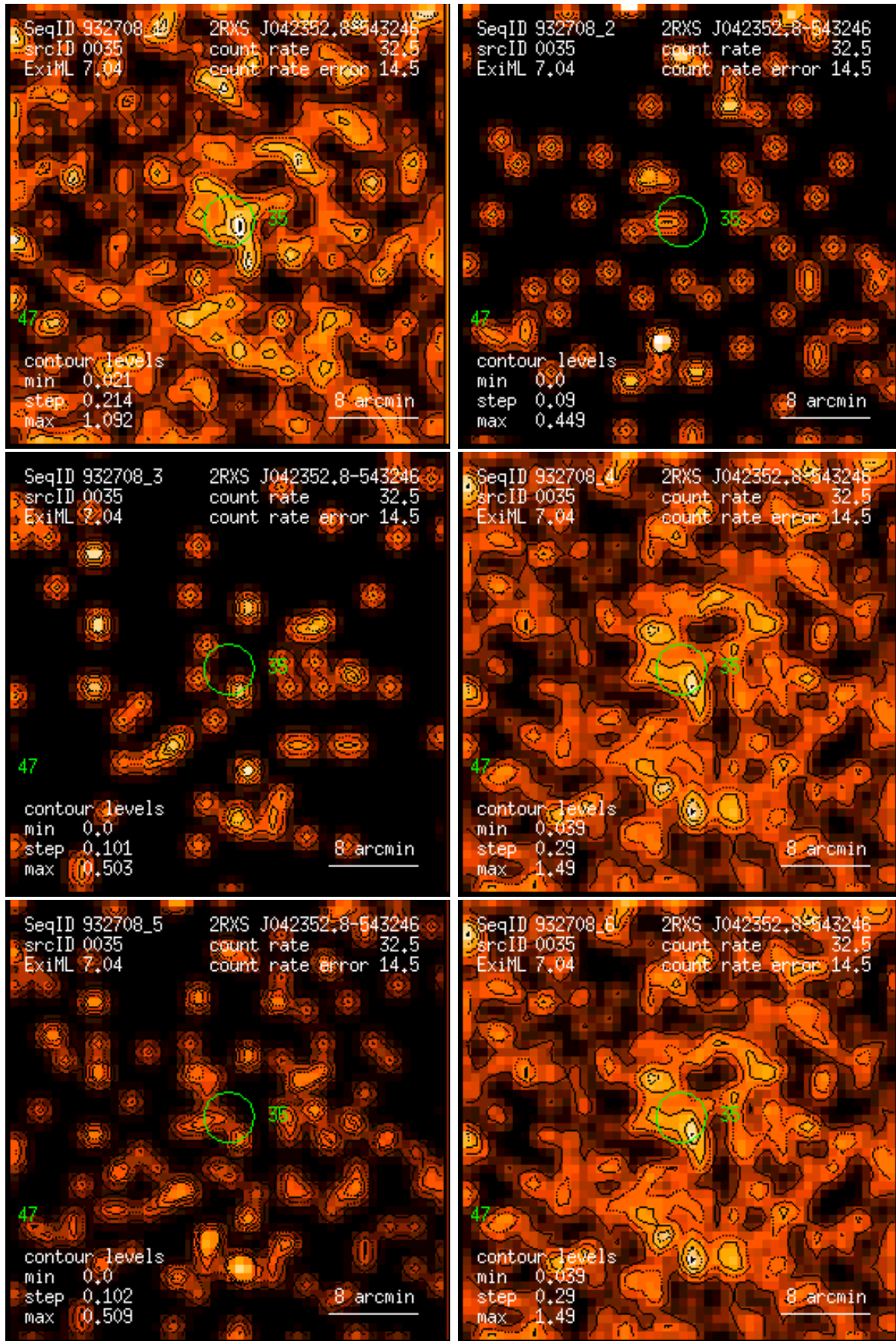
Figure 35: RASS 932708: detection 0035: band rate images, Gaussian filter: (1) PSPC channels 11 – 41, (2) 52 – 90, (3) 91 – 201, (4) 11 – 235, (5) 52 – 201, (6) 11 – 201. Broad band rates in counts/ks. Band rate contour levels in counts/ks/arcmin 2 .
