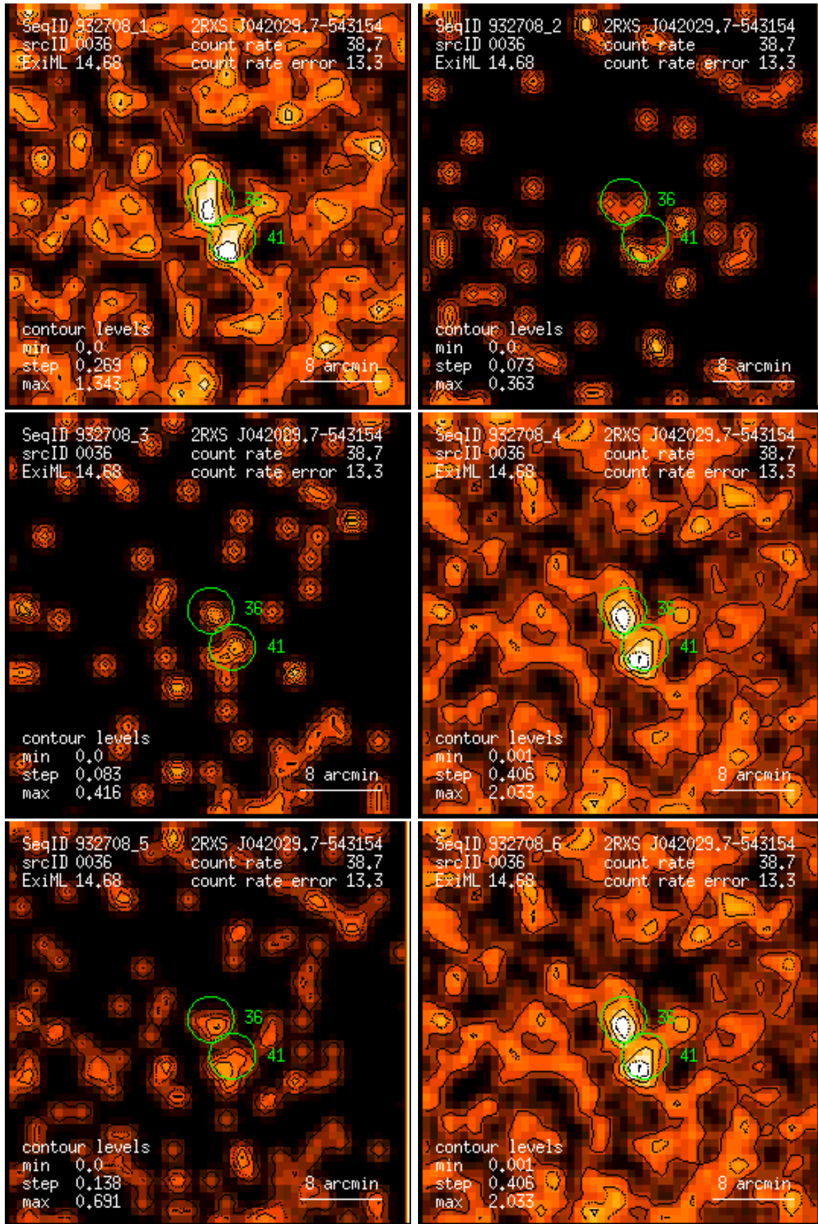
Figure 36: RASS 932708: detection 0036: band rate images, Gaussian filter: (1) PSPC channels 11 – 41, (2) 52 – 90, (3) 91 – 201, (4) 11 – 235, (5) 52 – 201, (6) 11 – 201. Broad band rates in counts/ks. Band rate contour levels in counts/ks/arcmin 2 .
