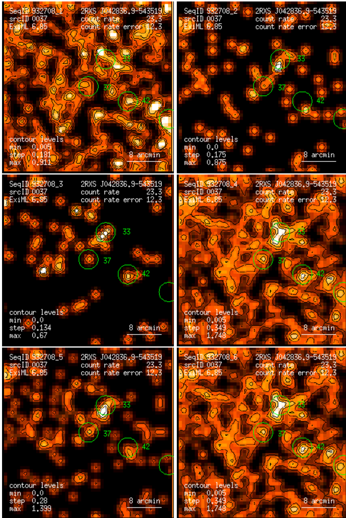
Figure 37: RASS 932708: detection 0037: band rate images, Gaussian filter: (1) PSPC channels 11 – 41, (2) 52 – 90, (3) 91 – 201, (4) 11 – 235, (5) 52 – 201, (6) 11 – 201. Broad band rates in counts/ks. Band rate contour levels in counts/ks/arcmin 2 .
