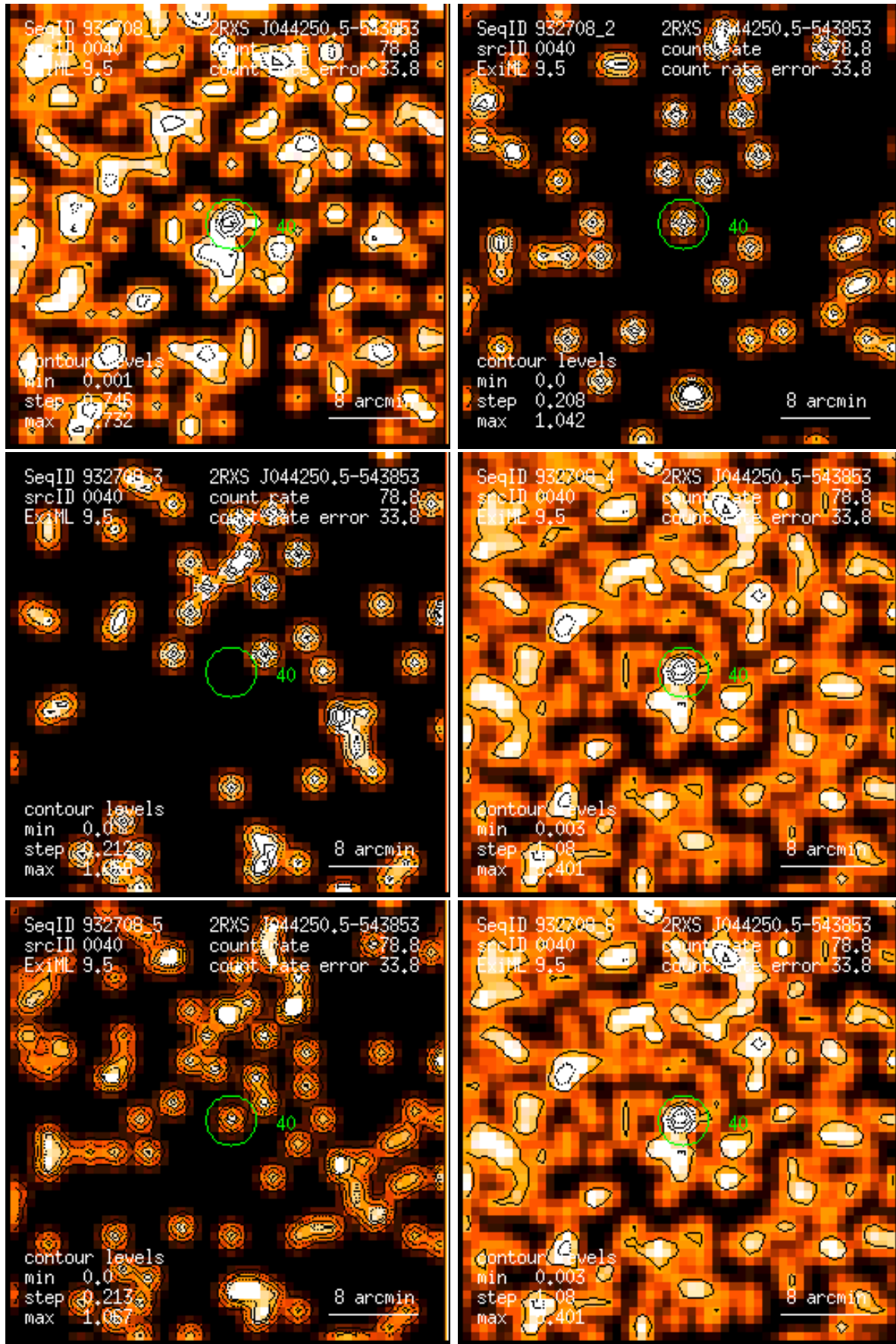
Figure 40: RASS 932708: detection 0040: band rate images, Gaussian filter: (1) PSPC channels 11 – 41, (2) 52 – 90, (3) 91 – 201, (4) 11 – 235, (5) 52 – 201, (6) 11 – 201. Broad band rates in counts/ks. Band rate contour levels in counts/ks/arcmin 2 .
