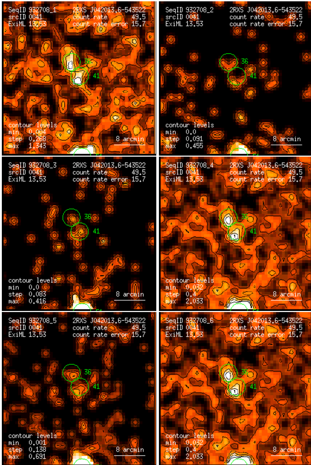
Figure 41: RASS 932708: detection 0041: band rate images, Gaussian filter: (1) PSPC channels 11 – 41, (2) 52 – 90, (3) 91 – 201, (4) 11 – 235, (5) 52 – 201, (6) 11 – 201. Broad band rates in counts/ks. Band rate contour levels in counts/ks/arcmin 2 .
