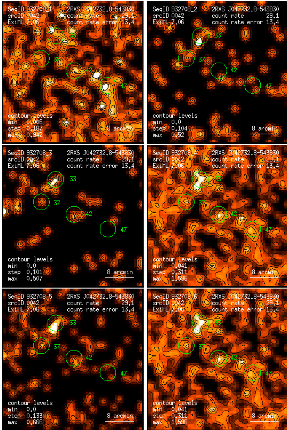
Figure 42: RASS 932708: detection 0042: band rate images, Gaussian filter: (1) PSPC channels 11 – 41, (2) 52 – 90, (3) 91 – 201, (4) 11 – 235, (5) 52 – 201, (6) 11 – 201. Broad band rates in counts/ks. Band rate contour levels in counts/ks/arcmin 2 .
