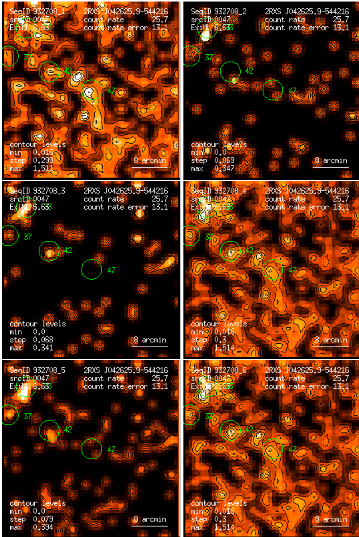
Figure 47: RASS 932708: detection 0047: band rate images, Gaussian filter: (1) PSPC channels 11 – 41, (2) 52 – 90, (3) 91 – 201, (4) 11 – 235, (5) 52 – 201, (6) 11 – 201. Broad band rates in counts/ks. Band rate contour levels in counts/ks/arcmin 2 .
