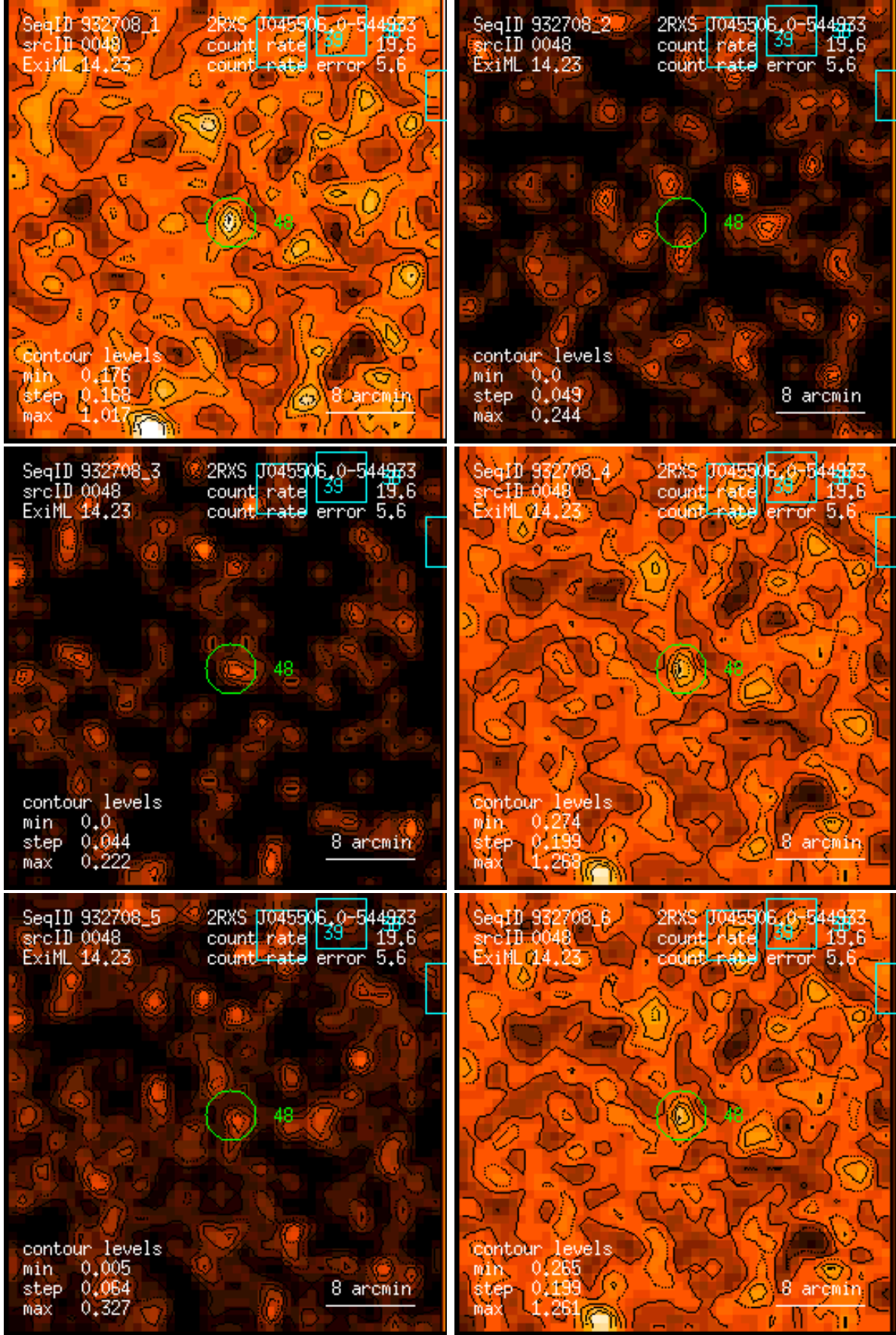
Figure 48: RASS 932708: detection 0048: band rate images, Gaussian filter: (1) PSPC channels 11 – 41, (2) 52 – 90, (3) 91 – 201, (4) 11 – 235, (5) 52 – 201, (6) 11 – 201. Broad band rates in counts/ks. Band rate contour levels in counts/ks/arcmin 2 .
