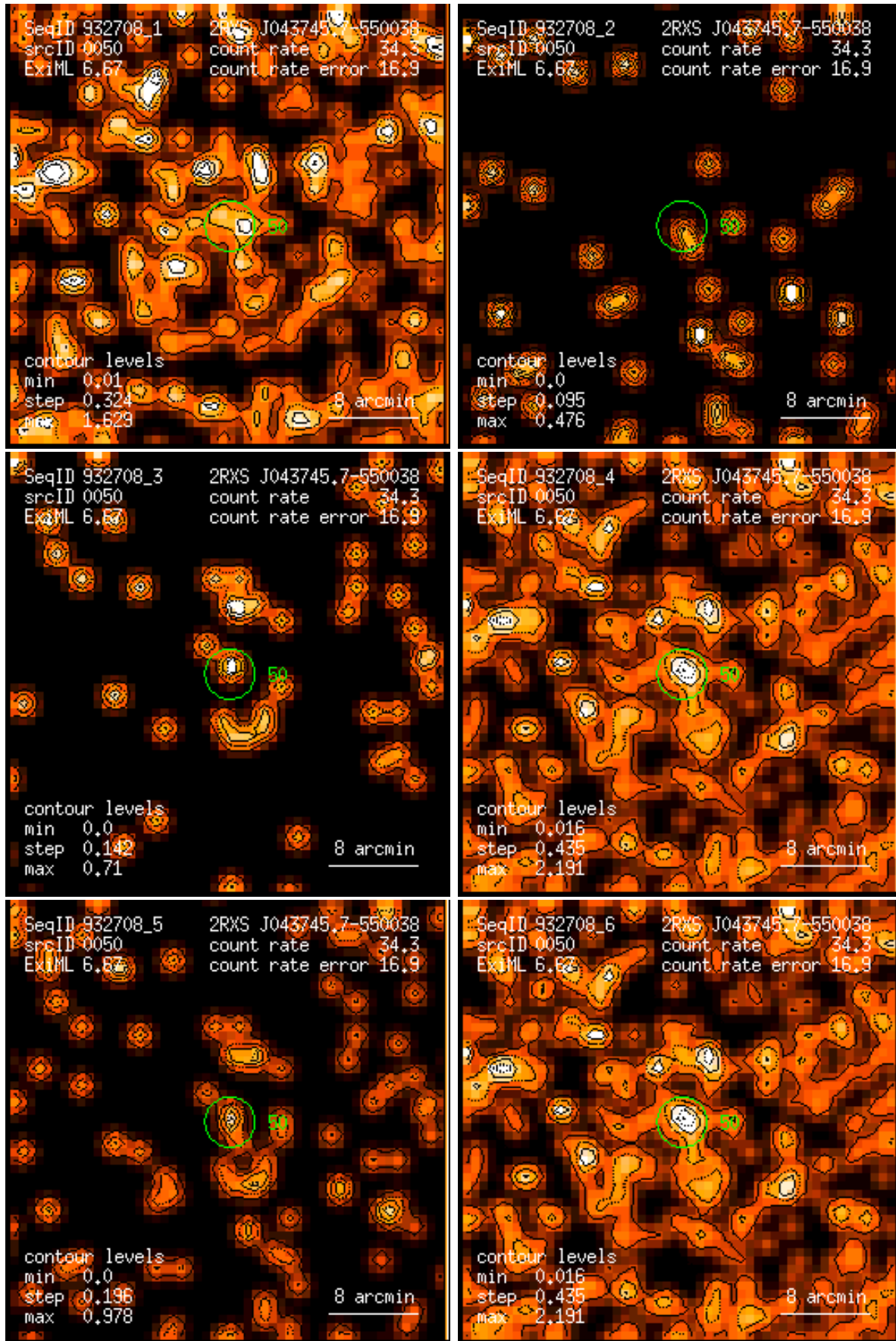
Figure 50: RASS 932708: detection 0050: band rate images, Gaussian filter: (1) PSPC channels 11 – 41, (2) 52 – 90, (3) 91 – 201, (4) 11 – 235, (5) 52 – 201, (6) 11 – 201. Broad band rates in counts/ks. Band rate contour levels in counts/ks/arcmin 2 .
