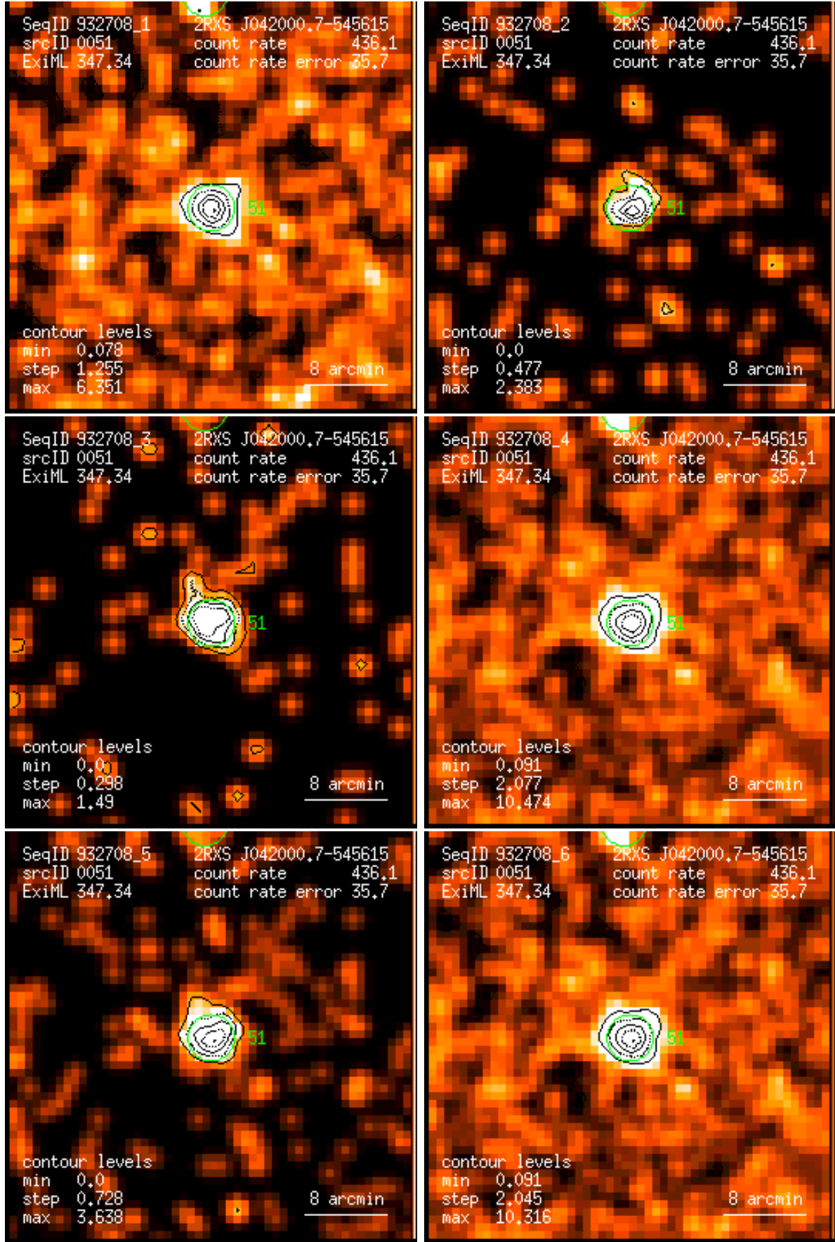
Figure 51: RASS 932708: detection 0051: band rate images, Gaussian filter: (1) PSPC channels 11 – 41, (2) 52 – 90, (3) 91 – 201, (4) 11 – 235, (5) 52 – 201, (6) 11 – 201. Broad band rates in counts/ks. Band rate contour levels in counts/ks/arcmin 2 .
