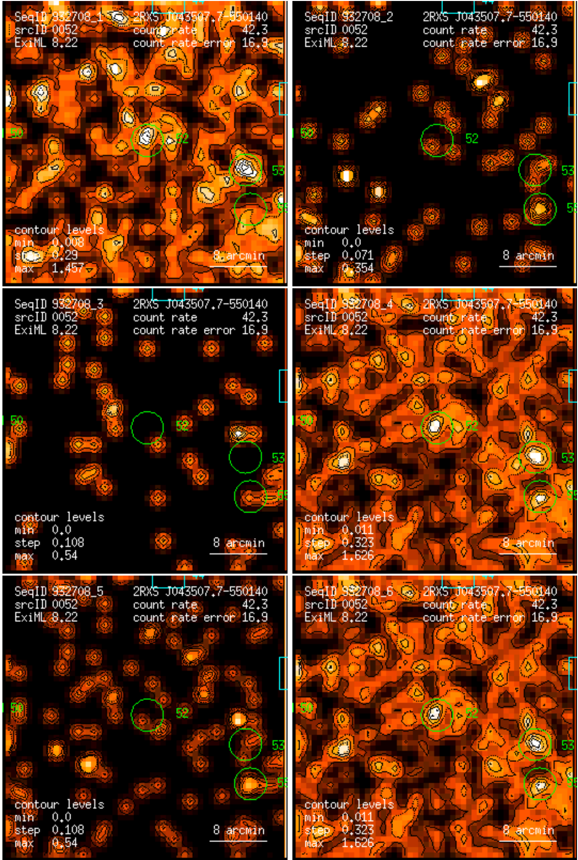
Figure 52: RASS 932708: detection 0052: band rate images, Gaussian filter: (1) PSPC channels 11 – 41, (2) 52 – 90, (3) 91 – 201, (4) 11 – 235, (5) 52 – 201, (6) 11 – 201. Broad band rates in counts/ks. Band rate contour levels in counts/ks/arcmin 2 .
