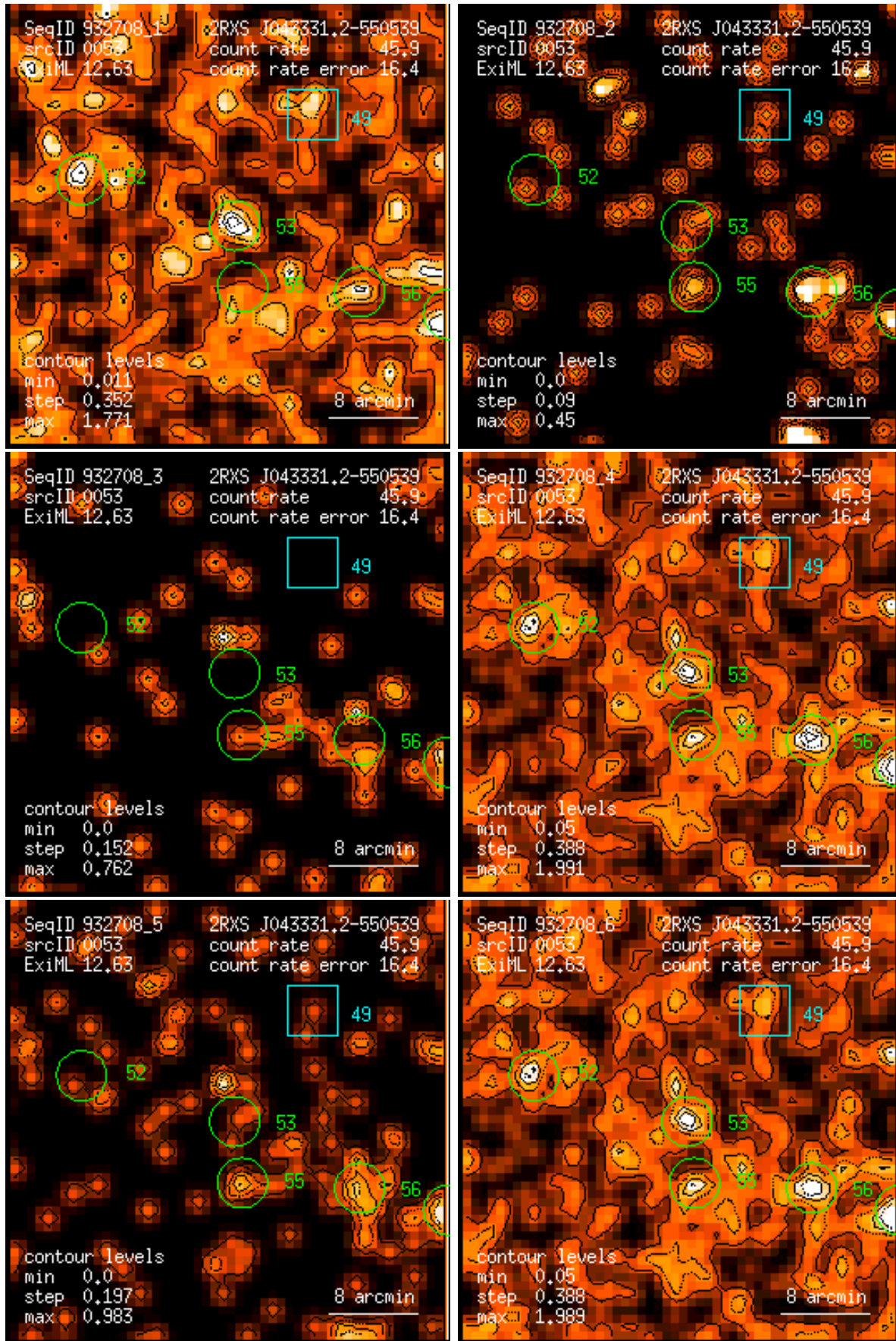
Figure 53: RASS 932708: detection 0053: band rate images, Gaussian filter: (1) PSPC channels 11 – 41, (2) 52 – 90, (3) 91 – 201, (4) 11 – 235, (5) 52 – 201, (6) 11 – 201. Broad band rates in counts/ks. Band rate contour levels in counts/ks/arcmin 2 .
