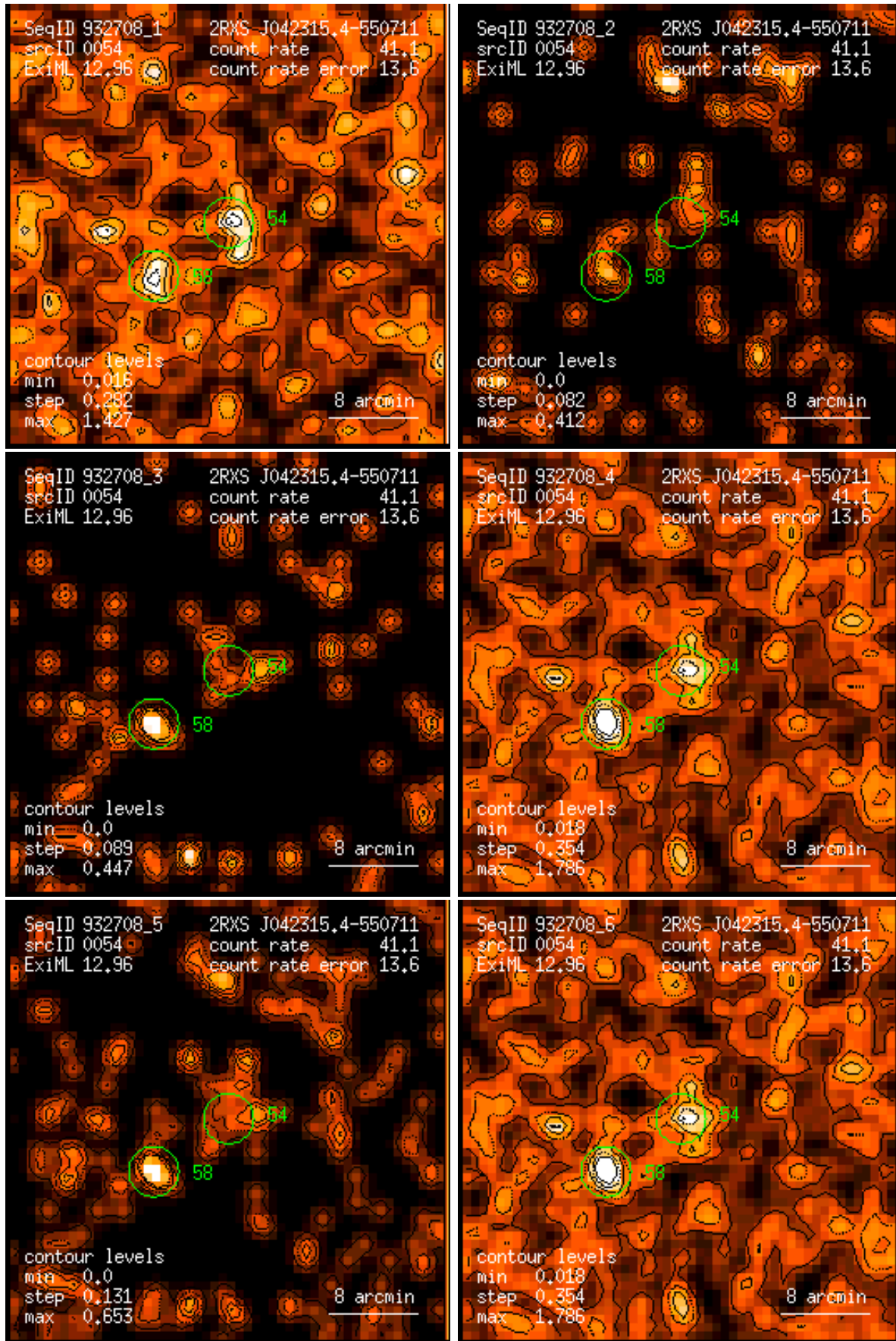
Figure 54: RASS 932708: detection 0054: band rate images, Gaussian filter: (1) PSPC channels 11 – 41, (2) 52 – 90, (3) 91 – 201, (4) 11 – 235, (5) 52 – 201, (6) 11 – 201. Broad band rates in counts/ks. Band rate contour levels in counts/ks/arcmin 2 .
