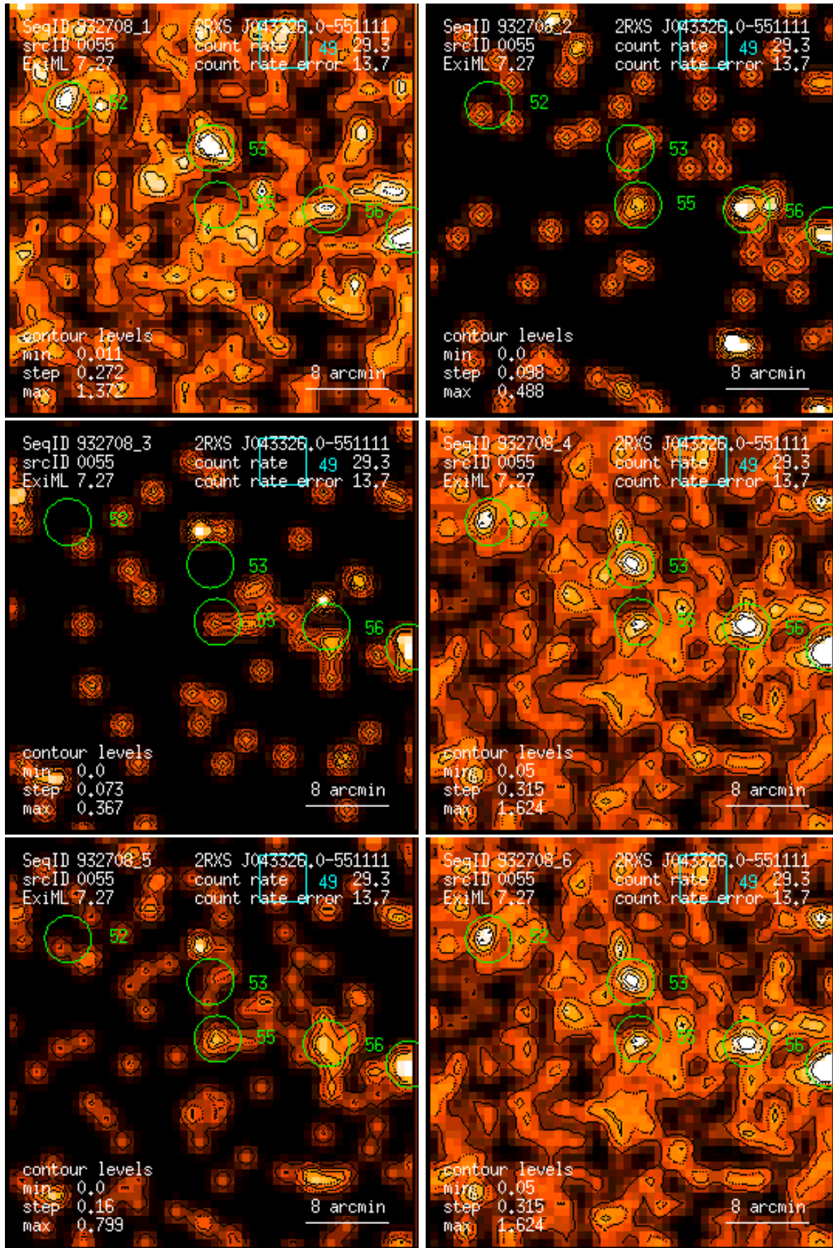
Figure 55: RASS 932708: detection 0055: band rate images, Gaussian filter: (1) PSPC channels 11 – 41, (2) 52 – 90, (3) 91 – 201, (4) 11 – 235, (5) 52 – 201, (6) 11 – 201. Broad band rates in counts/ks. Band rate contour levels in counts/ks/arcmin 2 .
