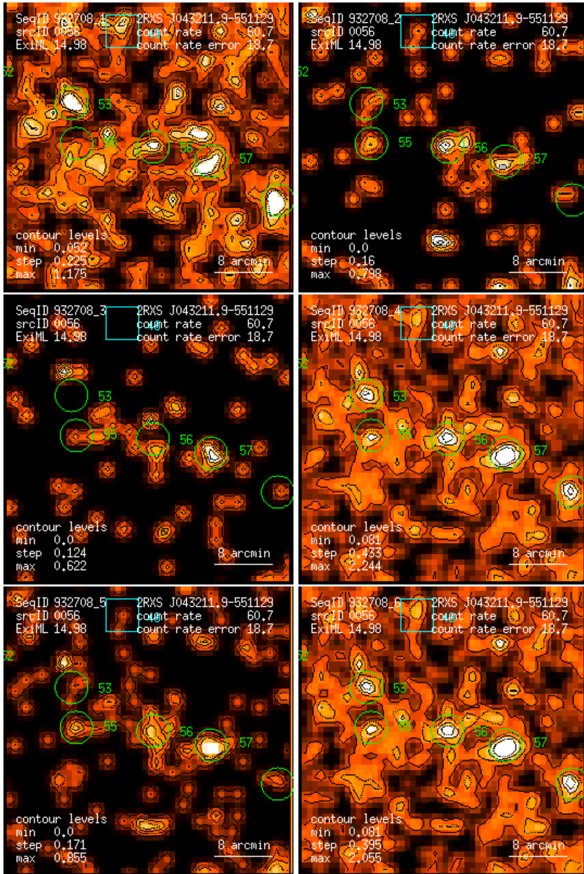
Figure 56: RASS 932708: detection 0056: band rate images, Gaussian filter: (1) PSPC channels 11 – 41, (2) 52 – 90, (3) 91 – 201, (4) 11 – 235, (5) 52 – 201, (6) 11 – 201. Broad band rates in counts/ks. Band rate contour levels in counts/ks/arcmin 2 .
