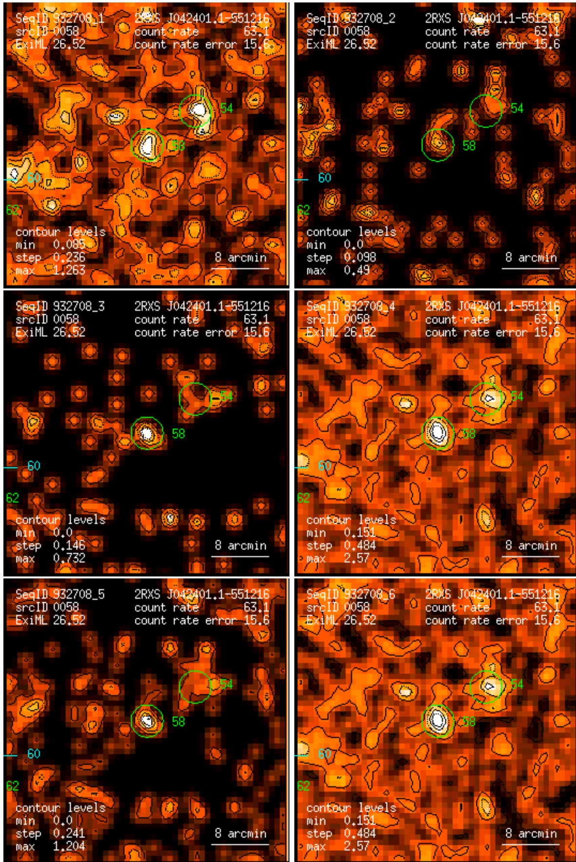
Figure 58: RASS 932708: detection 0058: band rate images, Gaussian filter: (1) PSPC channels 11 – 41, (2) 52 – 90, (3) 91 – 201, (4) 11 – 235, (5) 52 – 201, (6) 11 – 201. Broad band rates in counts/ks. Band rate contour levels in counts/ks/arcmin 2 .
