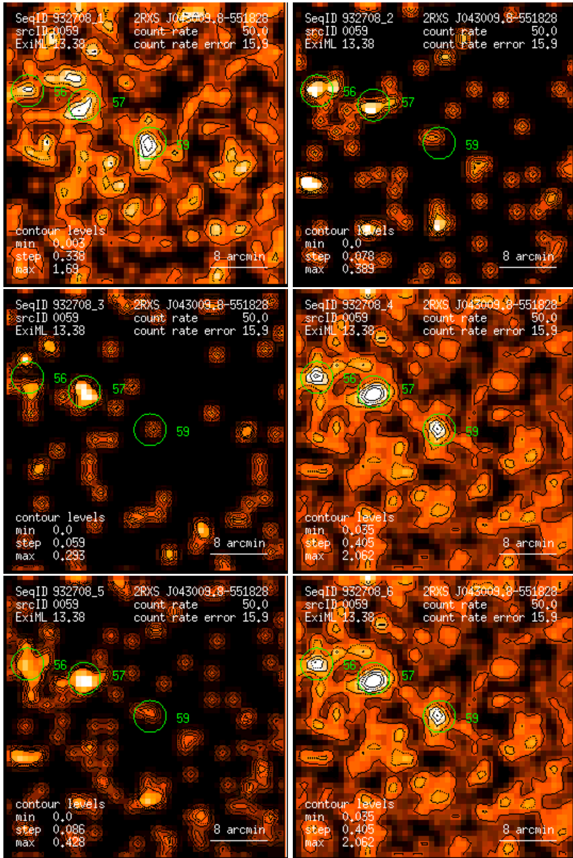
Figure 59: RASS 932708: detection 0059: band rate images, Gaussian filter: (1) PSPC channels 11 – 41, (2) 52 – 90, (3) 91 – 201, (4) 11 – 235, (5) 52 – 201, (6) 11 – 201. Broad band rates in counts/ks. Band rate contour levels in counts/ks/arcmin 2 .
