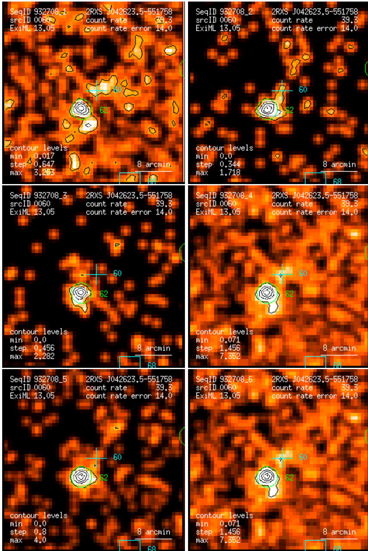
Figure 60: RASS 932708: detection 0060: band rate images, Gaussian filter: (1) PSPC channels 11 – 41, (2) 52 – 90, (3) 91 – 201, (4) 11 – 235, (5) 52 – 201, (6) 11 – 201. Broad band rates in counts/ks. Band rate contour levels in counts/ks/arcmin 2 .
