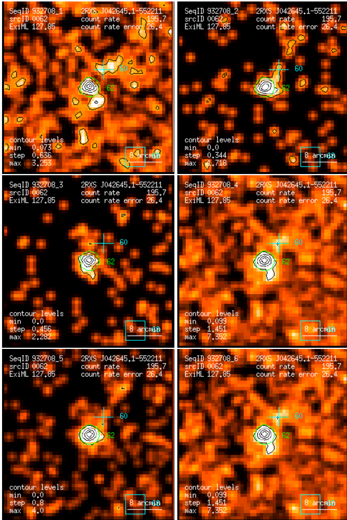
Figure 62: RASS 932708: detection 0062: band rate images, Gaussian filter: (1) PSPC channels 11 – 41, (2) 52 – 90, (3) 91 – 201, (4) 11 – 235, (5) 52 – 201, (6) 11 – 201. Broad band rates in counts/ks. Band rate contour levels in counts/ks/arcmin 2 .
