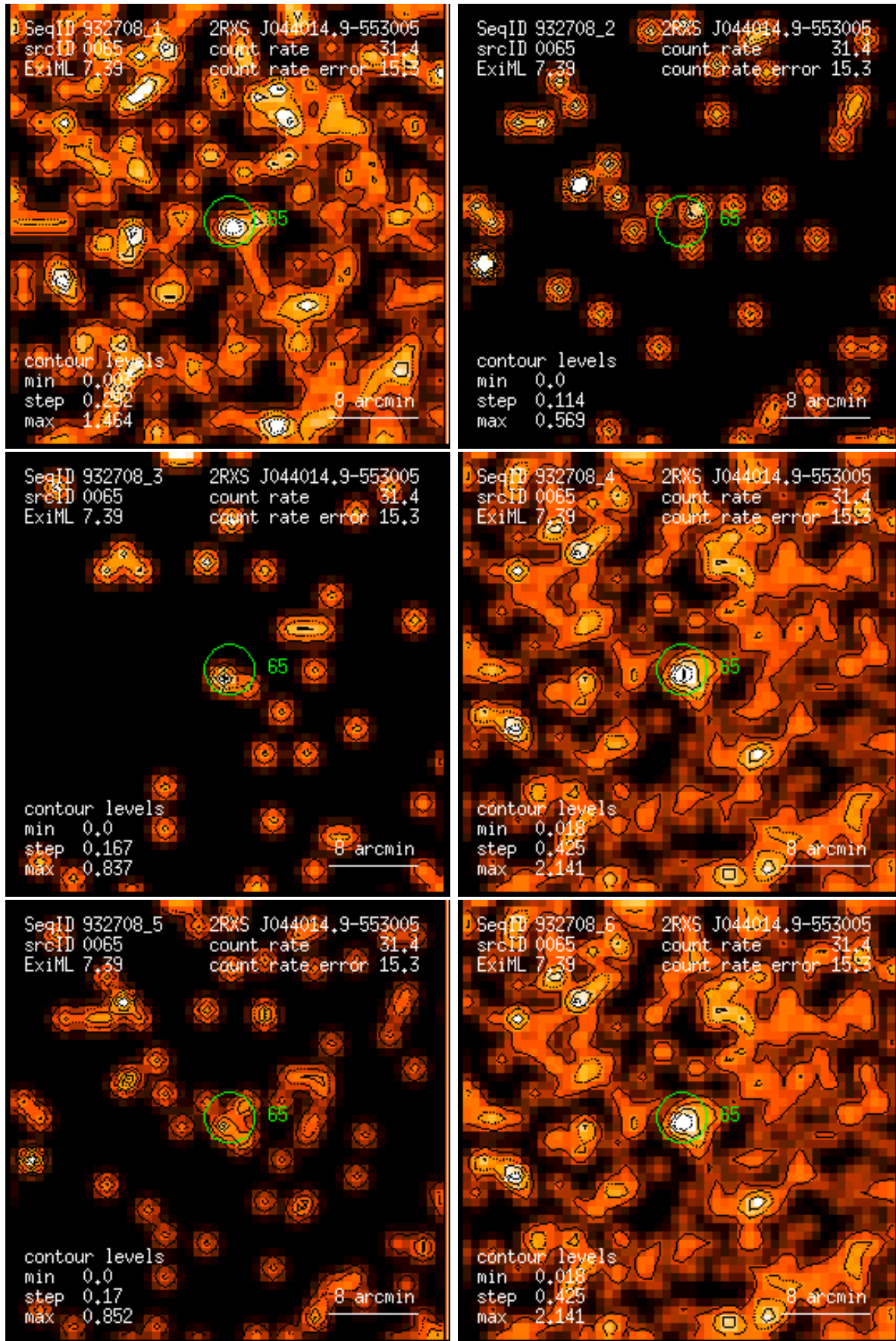
Figure 65: RASS 932708: detection 0065: band rate images, Gaussian filter: (1) PSPC channels 11 – 41, (2) 52 – 90, (3) 91 – 201, (4) 11 – 235, (5) 52 – 201, (6) 11 – 201. Broad band rates in counts/ks. Band rate contour levels in counts/ks/arcmin 2 .
